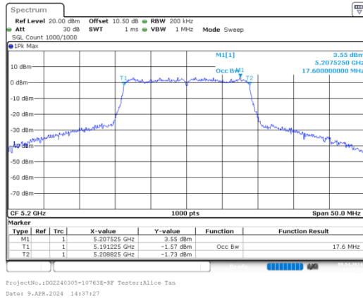
n20_5200MHz_Chain 0
