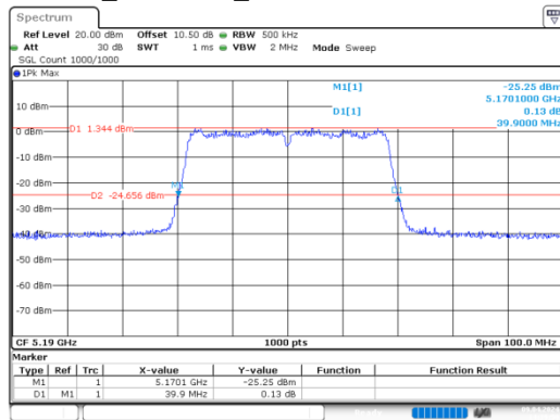
n40_5190MHz_Chain 0 39.900 MHz
