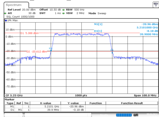
n40_5230MHz_Chain 0 39.900 MHz
