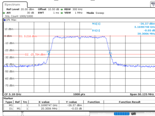
ac20_5180MHz_Chain 0
