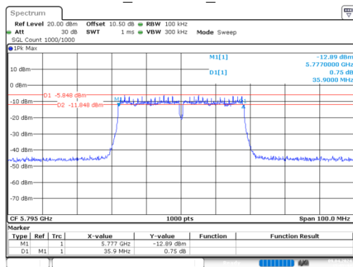
ac40_5795MHz_Chain 0
