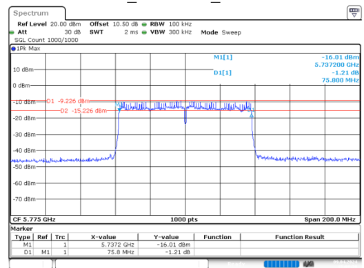
ac80_5775MHz_Chain 0
