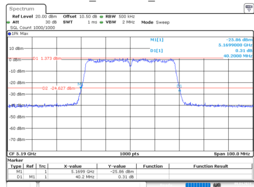
ac40_5190MHz_Chain 0
