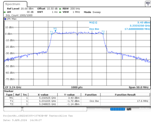
n20_5240MHz_Chain 0
