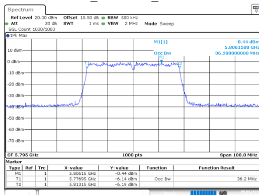
ac40_5795MHz_Chain 0
