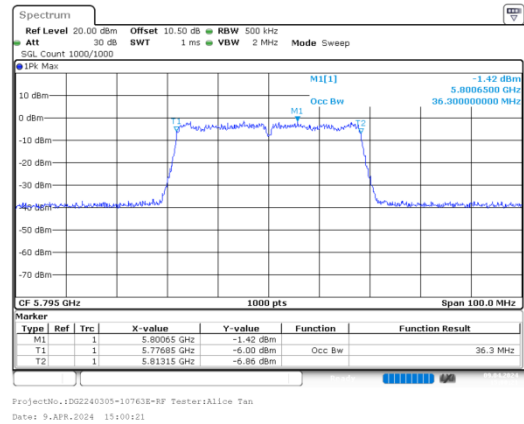
n40_5795MHz_Chain 0
