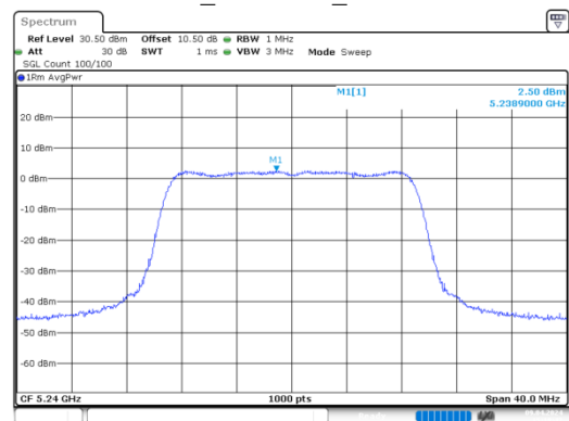
ac20_5240MHz_Chain 1
