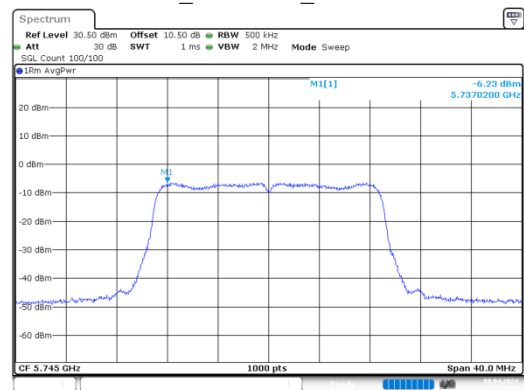
n20_5745MHz_Chain 1
