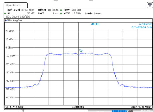
ac20_5745MHz_Chain 1
