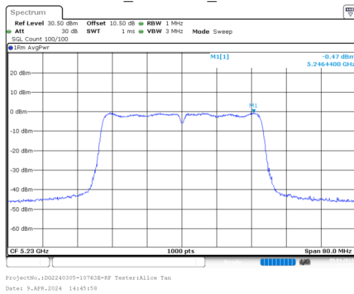
ac40_5230MHz_Chain 0
