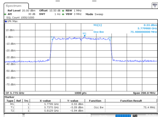
ac80_5775MHz_Chain 0
