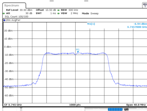
n20_5745MHz_Chain 0
