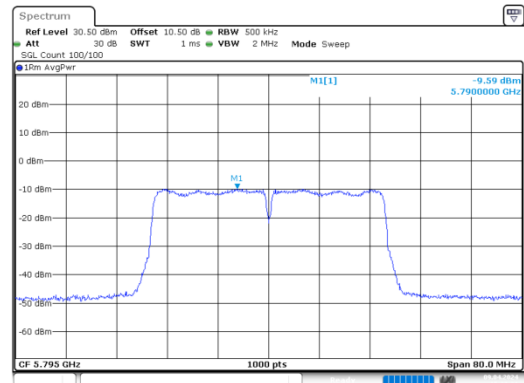
n40_5795MHz_Chain 1
