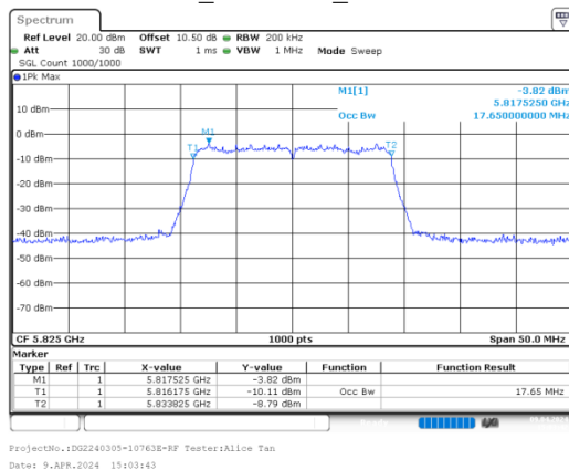
ac20_5825MHz_Chain 0
