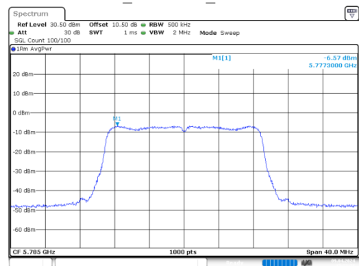
n20_5785MHz_Chain 1
