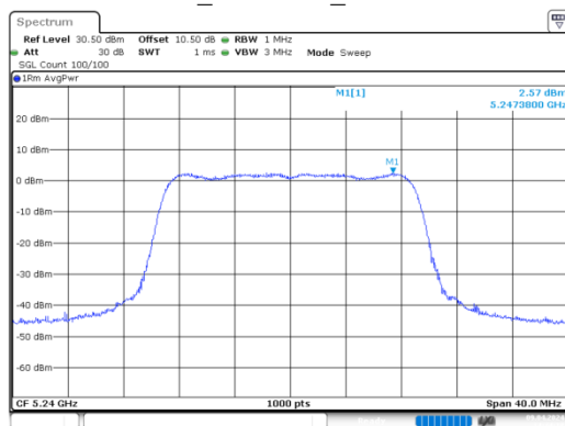
ac20_5240MHz_Chain 0
