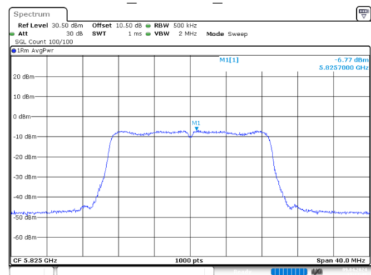
n20_5825MHz_Chain 1
