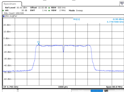
ac40_5795MHz_Chain 0
