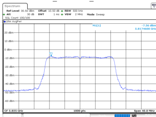
n20_5825MHz_Chain 0
