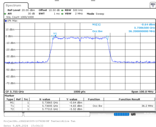
ac40_5755MHz_Chain 0
