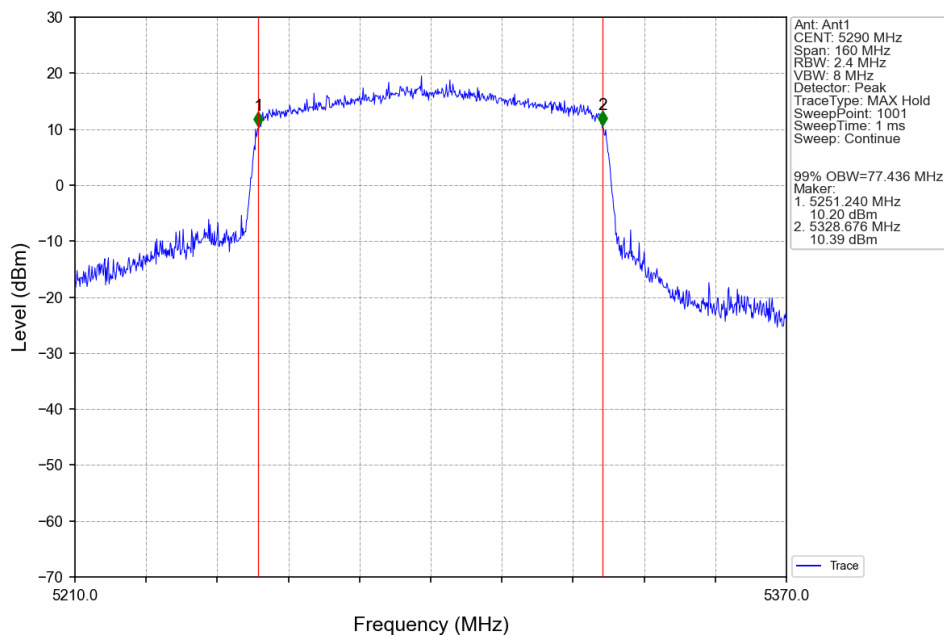
802.11ax(HEW80)_MCH_5290MHz_SU_/_Ant1_NTNV
