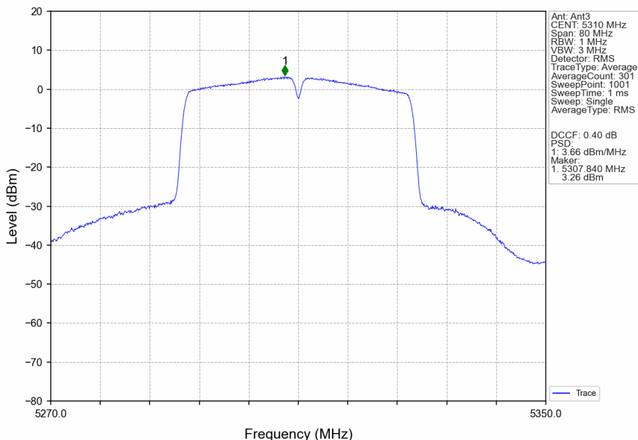
802.11n(HT40)_HCH_5310MHz_MIMO_NTNV
