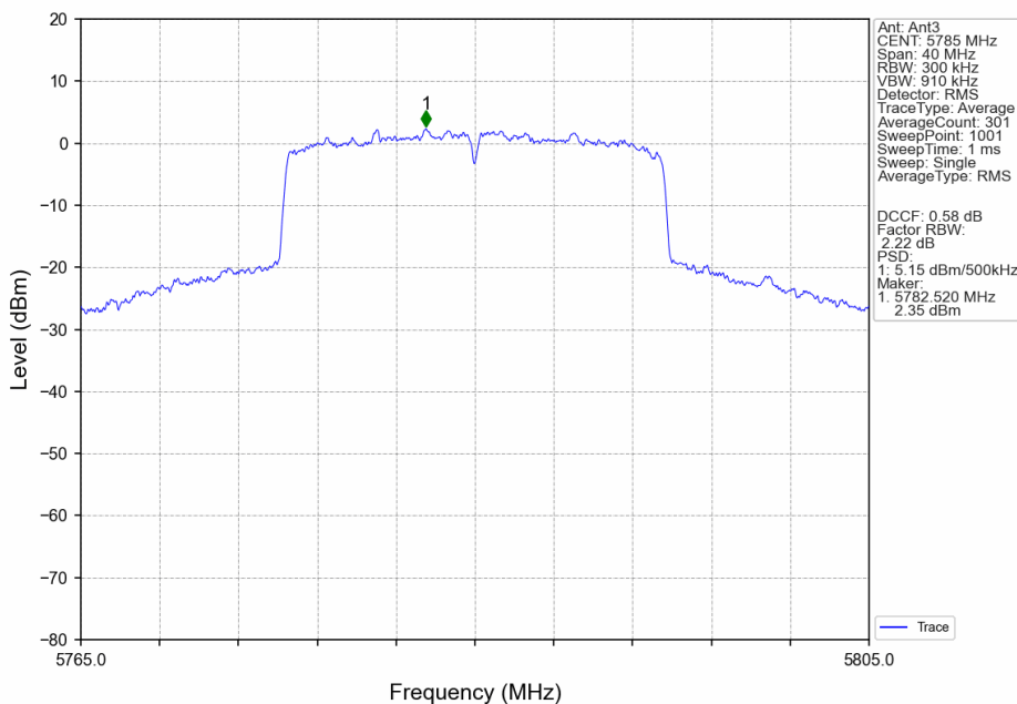
802.11ax(HEW20)_MCH_5785MHz_SU_/_Ant3_NTNV
