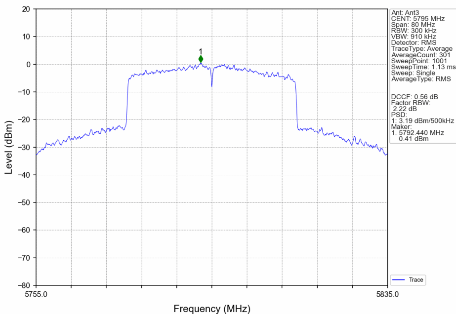
802.11be(EHT40)_HCH_5795MHz_SU_/_MIMO_NTNV
