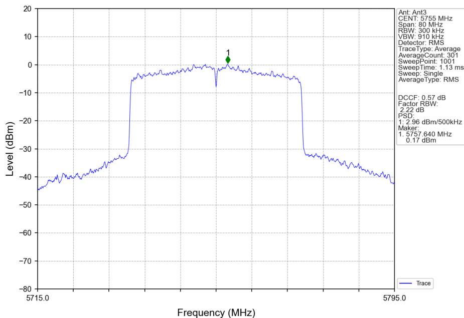
802.11ax(HEW40)_LCH_5755MHz_SU_ / _Ant3_NTNV
