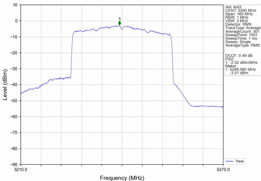
802.11ax(HEW80)_MCH_5290MHz_SU_/_Ant3_NTNV
