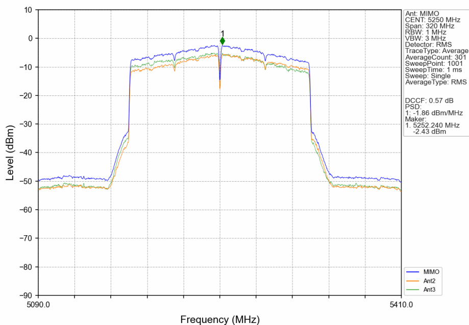
802.11ax(HEW160)_MCH_5250MHz_SU_/_MIMO_NTNV
