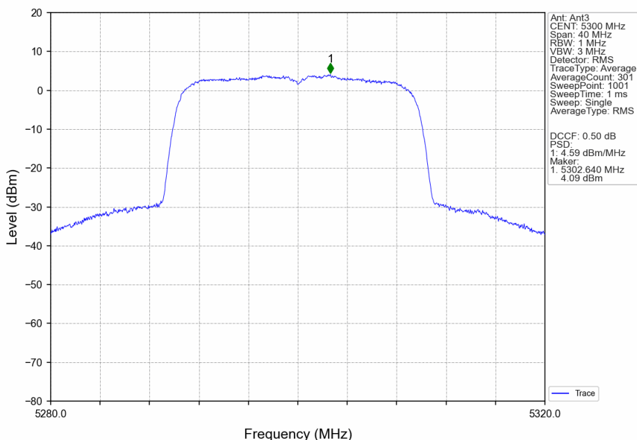
802.11ax(HEW20)_MCH_5300MHz_SU_/_MIMO_NTNV
