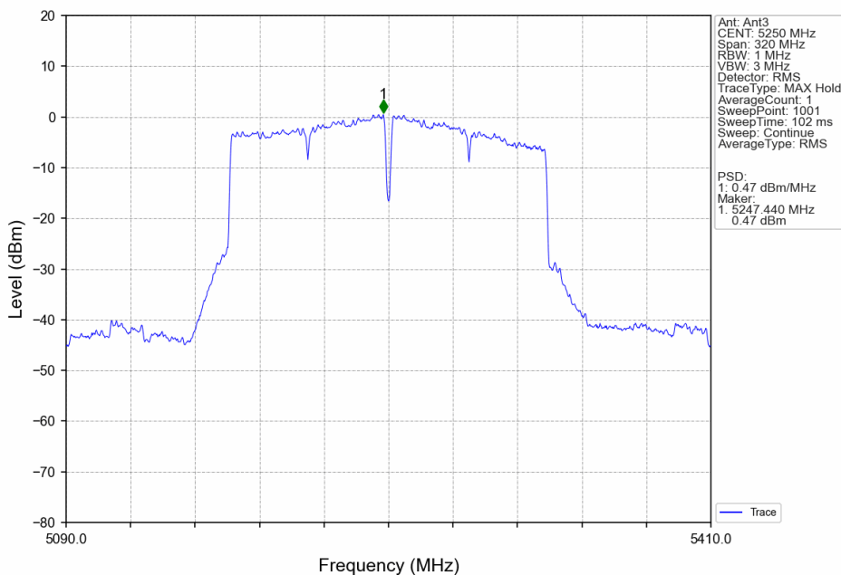
802.11ac(VHT160)_MCH_5250MHz_Ant3_NTNV
