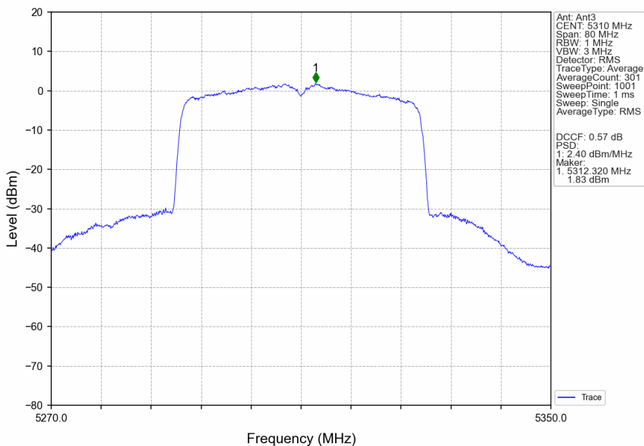
802.11ax(HEW40)_HCH_5310MHz_SU_/_Ant3_NTNV
