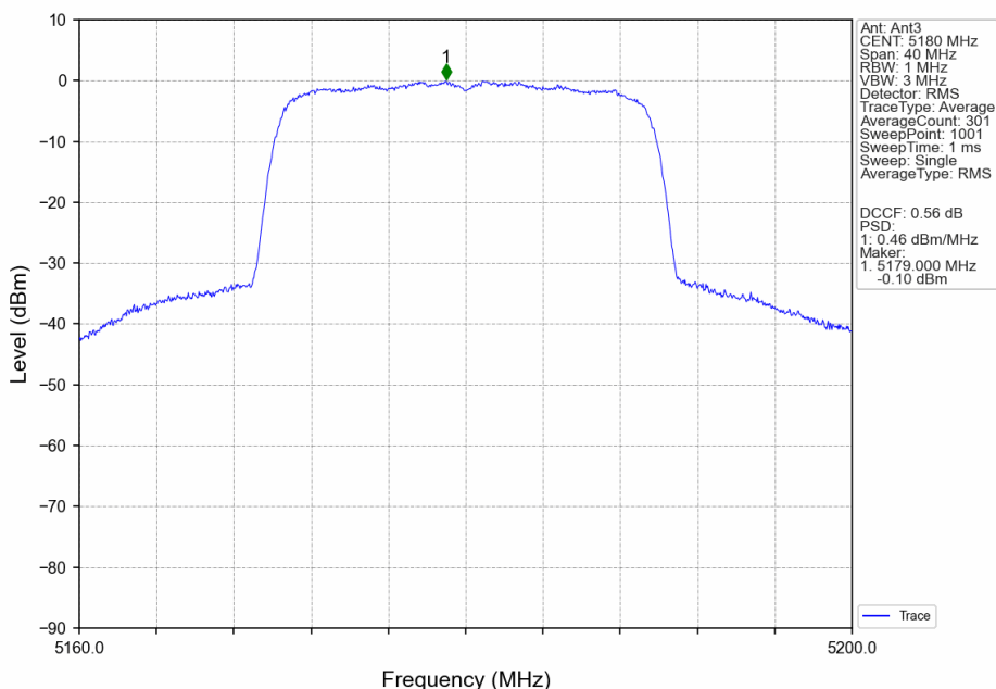
802.11ax(HEW20)_LCH_5180MHz_SU_ / _MIMO_NTNV
