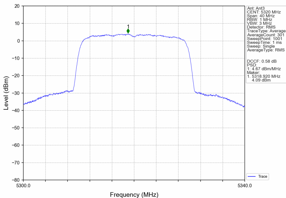
802.11ax(HEW20)_HCH_5320MHz_SU_/_Ant3_NTNV
