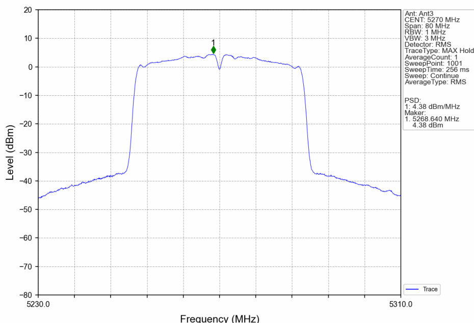
802.11ac(VHT40)_LCH_5270MHz_Ant3_NTNV
