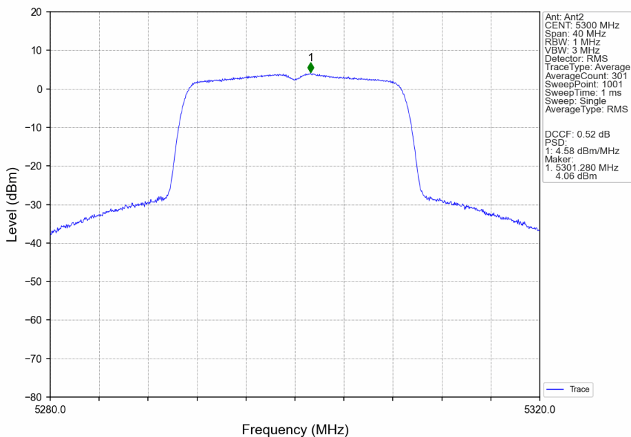
802.11ac(VHT20)_MCH_5300MHz_Ant2_NTNV
