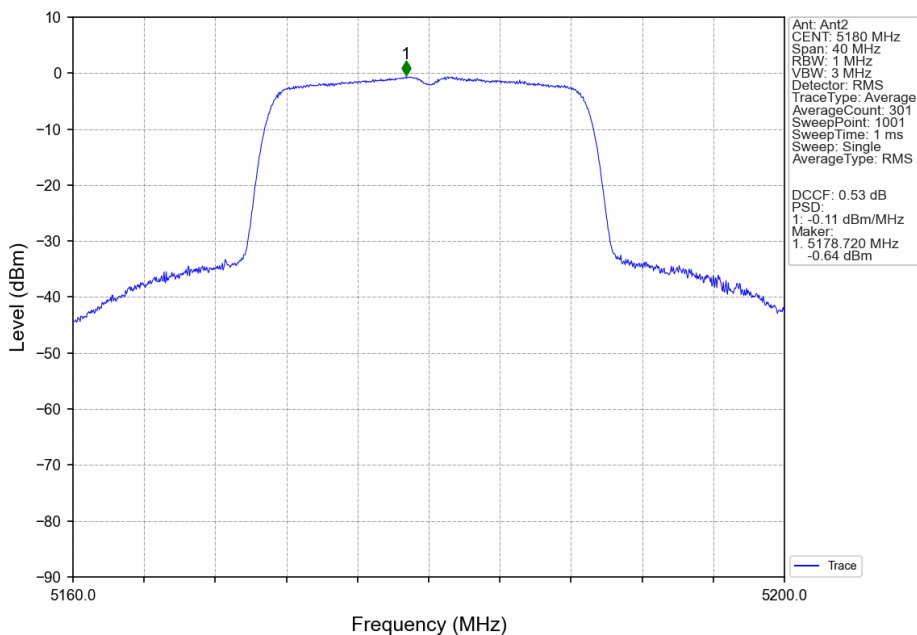
802.11ac(VHT20)_LCH_5180MHz_Ant2_NTNV
