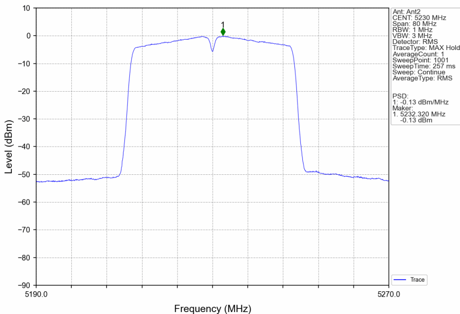
802.11ac(VHT40)_HCH_5230MHz_MIMO_NTNV
