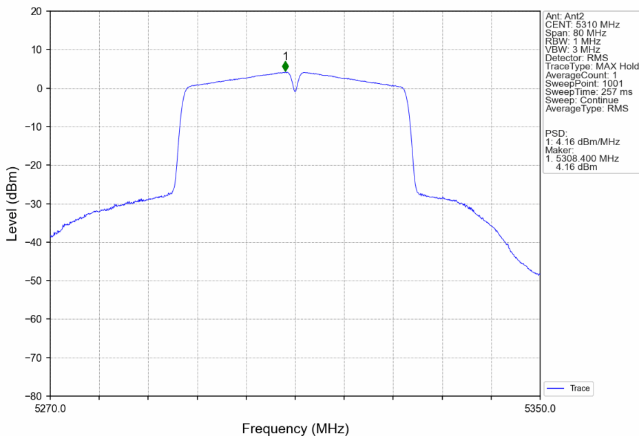
802.11ac(VHT40)_HCH_5310MHz_MIMO_NTNV
