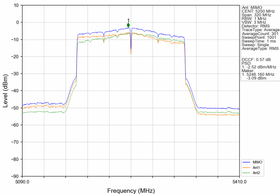
802.11ax(HEW160)_MCH_5250MHz_SU_/_MIMO_NTNV
