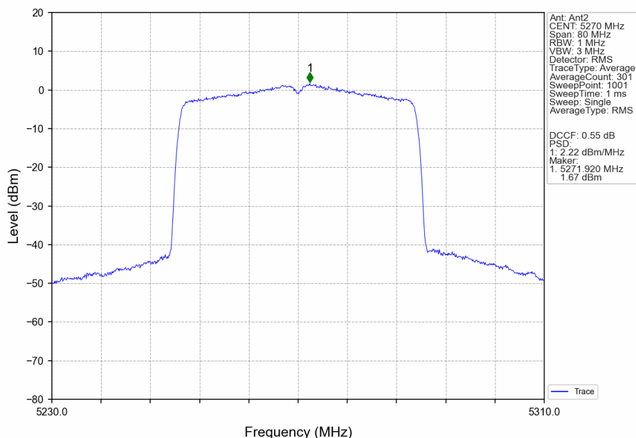
802.11ax(HEW40)_LCH_5270MHz_SU_ / _MIMO_NTNV
