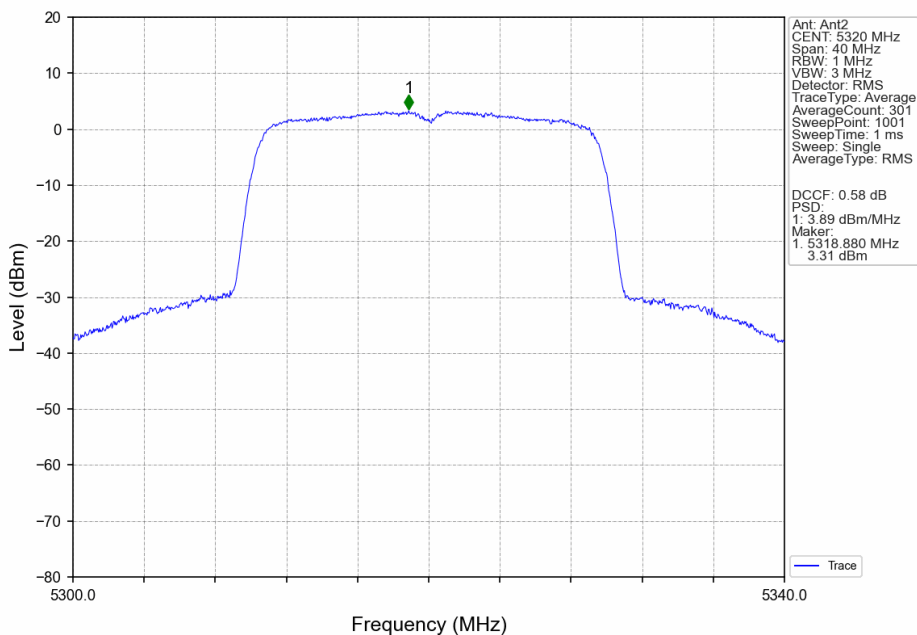
802.11ax(HEW20)_HCH_5320MHz_SU_/_Ant2_NTNV
