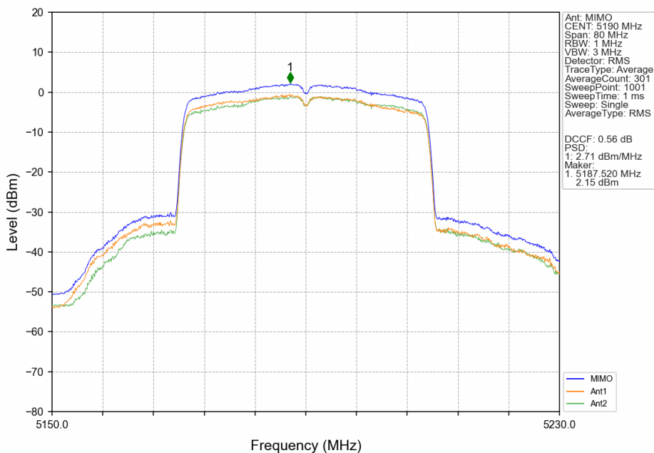
802.11ax(HEW40)_LCH_5190MHz_SU_ / _MIMO_NTNV
