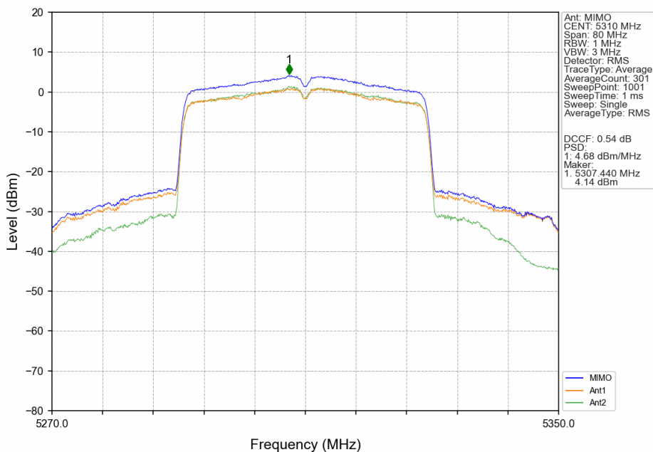
802.11be(EHT40)_HCH_5310MHz_SU_/_MIMO_NTNV
