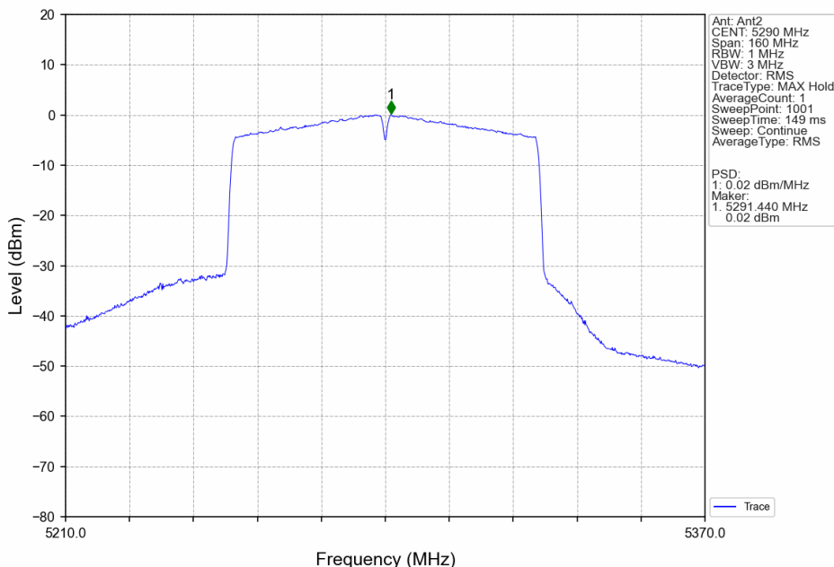
802.11ac(VHT80)_MCH_5290MHz_MIMO_NTNV
