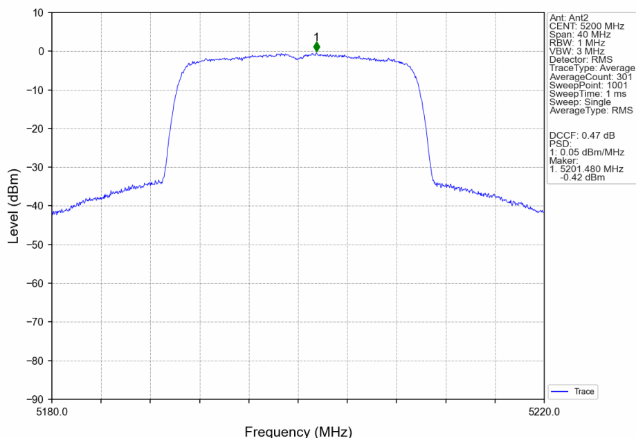
802.11be(EHT20)_MCH_5200MHz_SU_/_MIMO_NTNV
