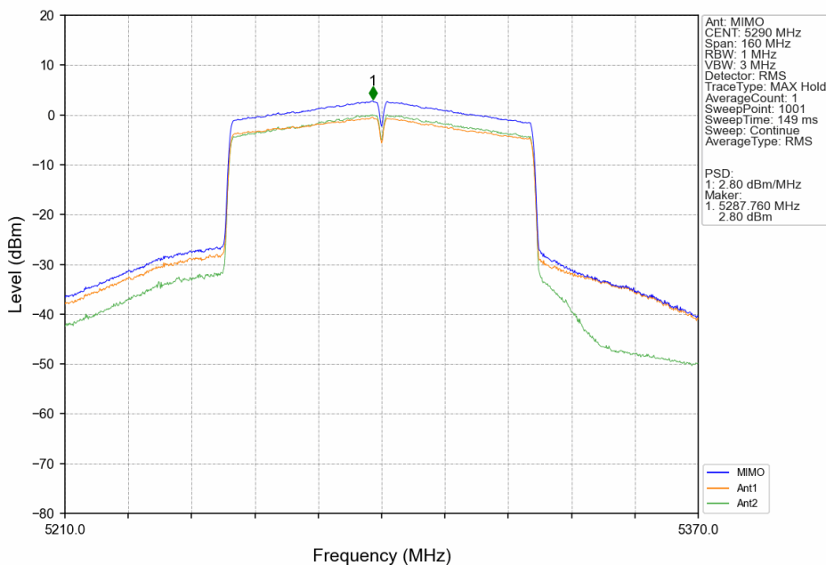
802.11ac(VHT80)_MCH_5290MHz_MIMO_NTNV
