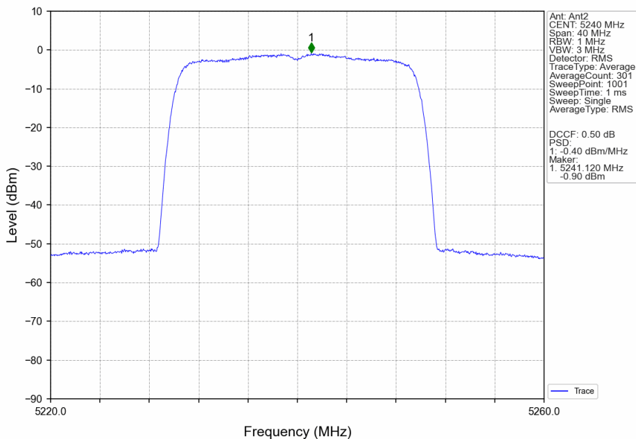
802.11ax(HEW20)_HCH_5240MHz_SU_/_MIMO_NTNV
