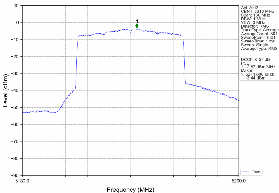
802.11ax(HEW80)_MCH_5210MHz_SU_/_MIMO_NTNV
