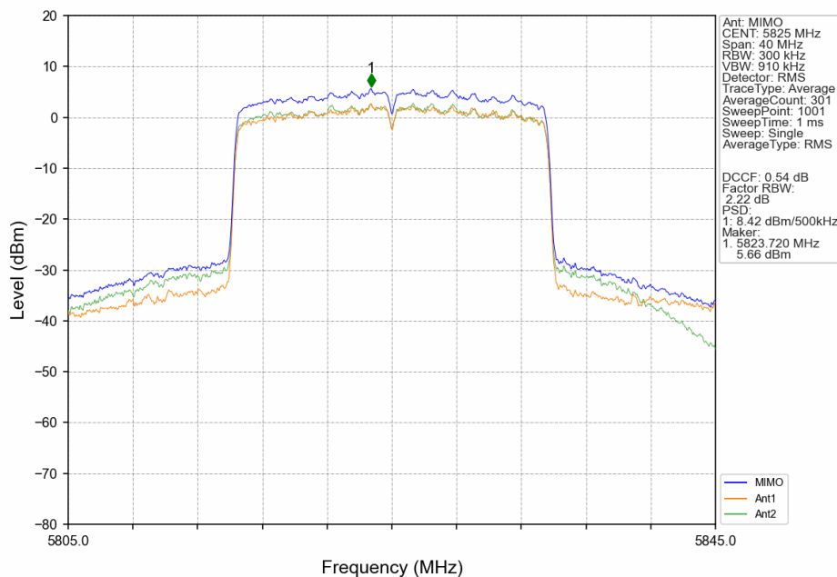
802.11be(EHT20)_HCH_5825MHz_SU_ / _MIMO_NTNV
