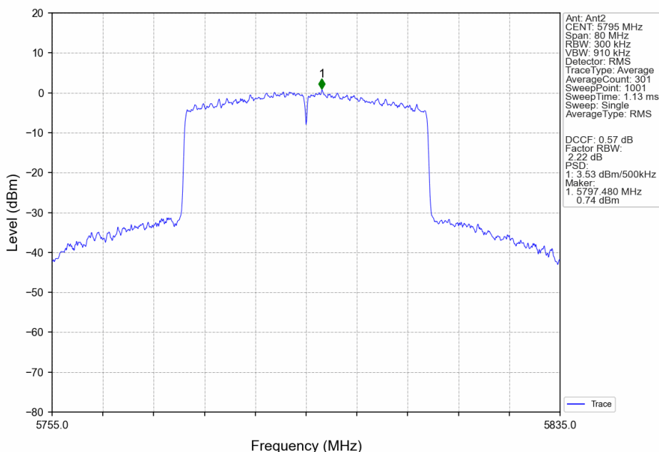
802.11ax(HEW40)_HCH_5795MHz_SU_/_MIMO_NTNV
