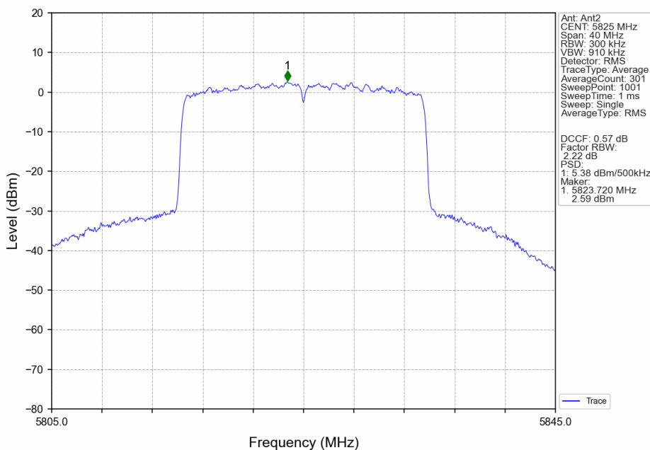
802.11ax(HEW20)_HCH_5825MHz_SU_/_MIMO_NTNV
