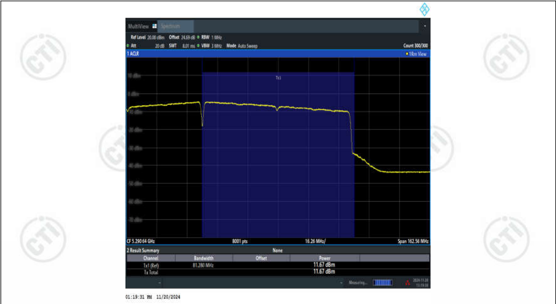
11BE160SISO-Ant2-5250_UNII-2A-TPC_H-PASS
