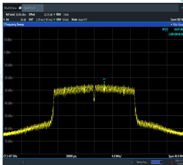
11N20MIMO-Ant1-2437-PASS
