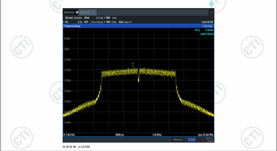
11G-Ant2-2462-PASS
