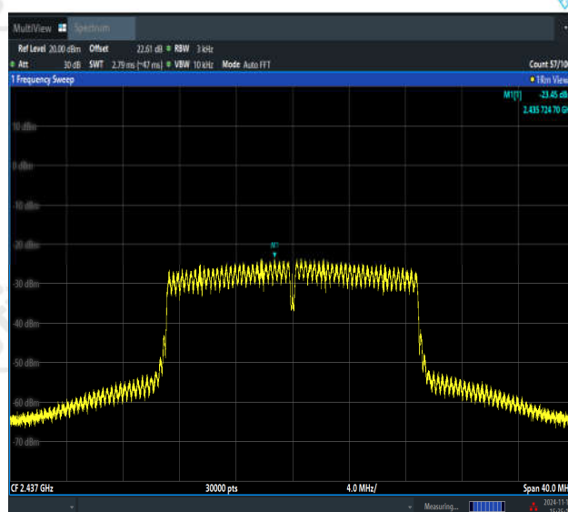
11N20MIMO-Ant2-2437-PASS
