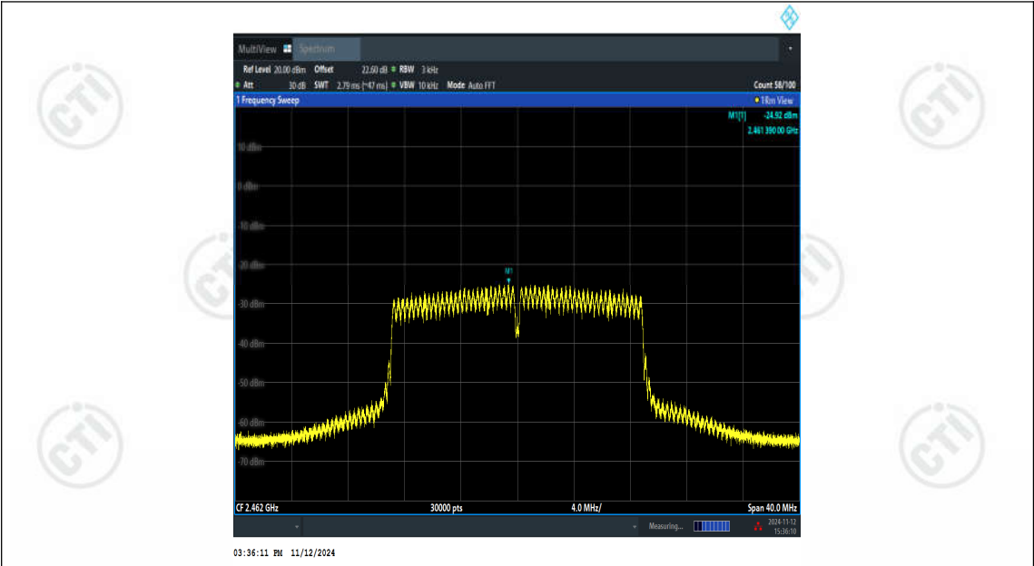
11N20MIMO-Ant1-2462-PASS
