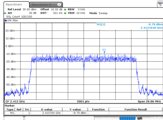
ax20_2412MHz_RU_Full_Chain 1
