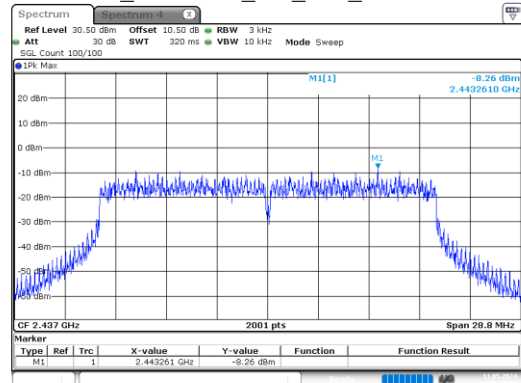
ax20_2437MHz_RU_Full_Chain 1
