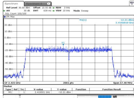
ax40_2422MHz_RU_Full_Chain 1
