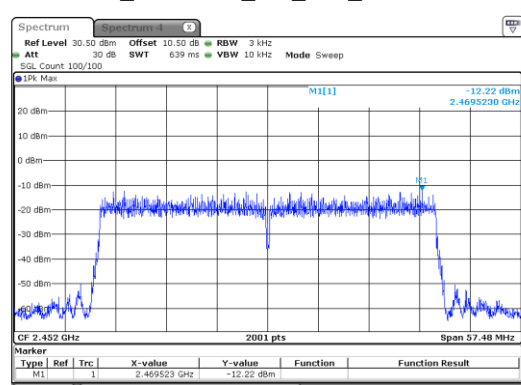
ax40_2452MHz_RU_Full_Chain 1
