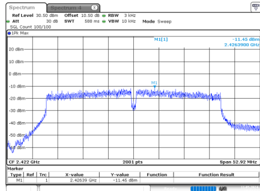
n40_2422MHz_Chain 1
