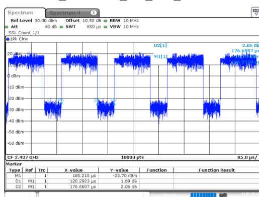
ax20_2437MHz_RU_Full_Chain 0
