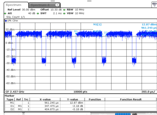
n40_2437MHz_Chain 0
