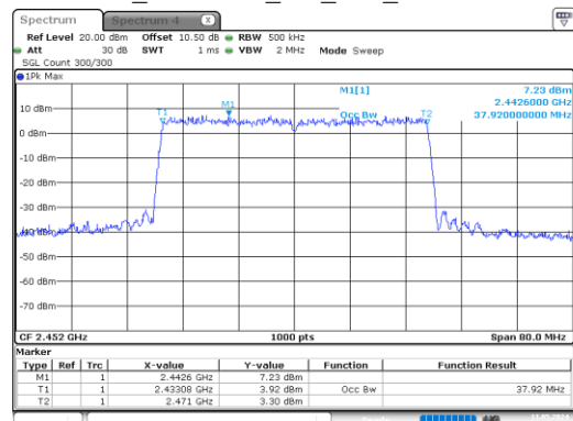
ax40_2452MHz_RU_Full_Chain 0
