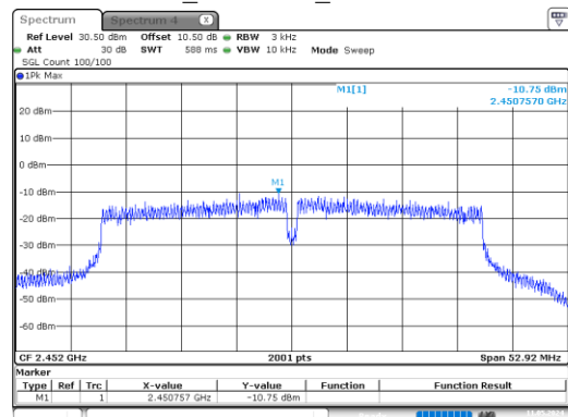
n40_2452MHz_Chain 1
