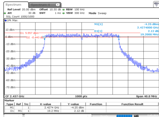
ax20_2437MHz_RU_Full_Chain 0
