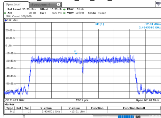
ax40_2437MHz_RU_Full_Chain 1
