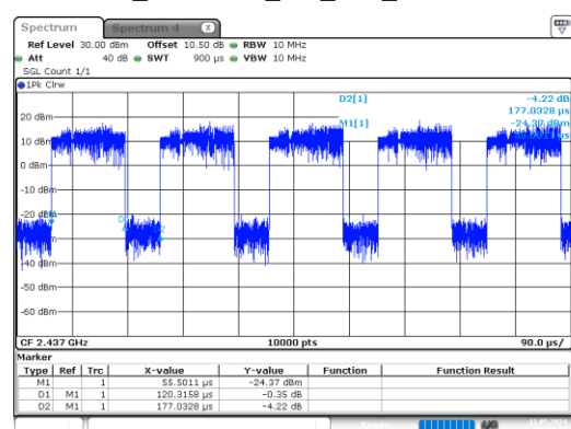
ax40_2437MHz_RU_Full_Chain 0
