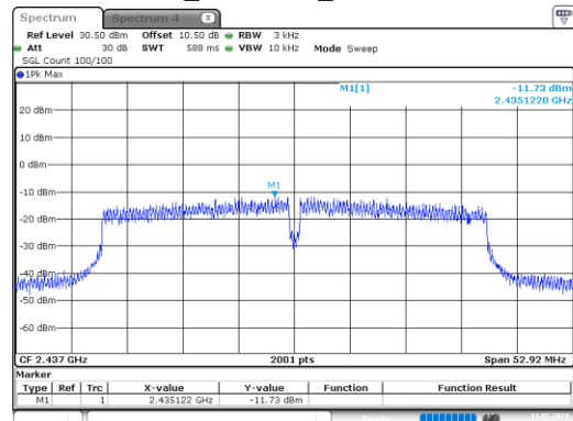
n40_2437MHz_Chain 1
