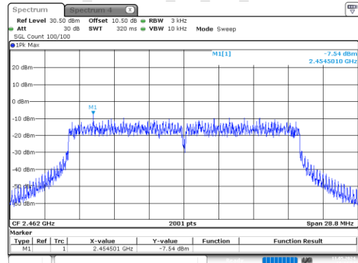
ax20_2462MHz_RU_Full_Chain 1
