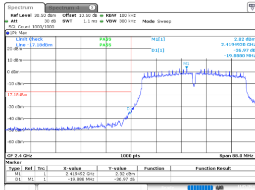
n40_2422MHz_Chain 0
