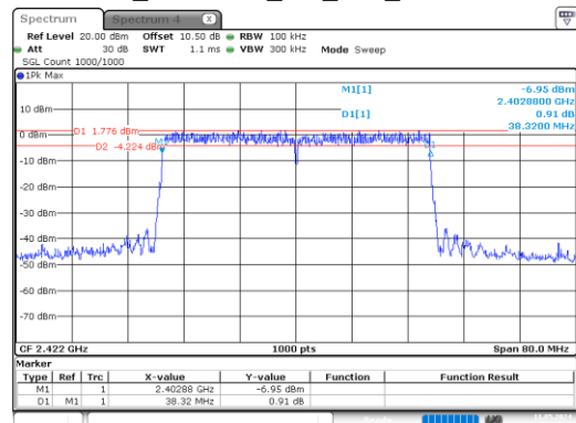
ax40_2422MHz_RU_Full_Chain 0
