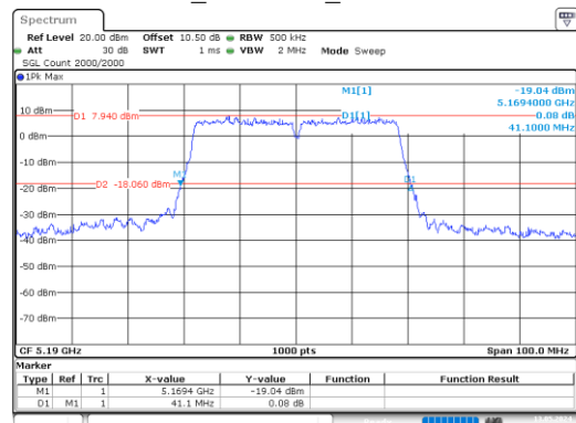
ac40_5190MHz_Chain 0
