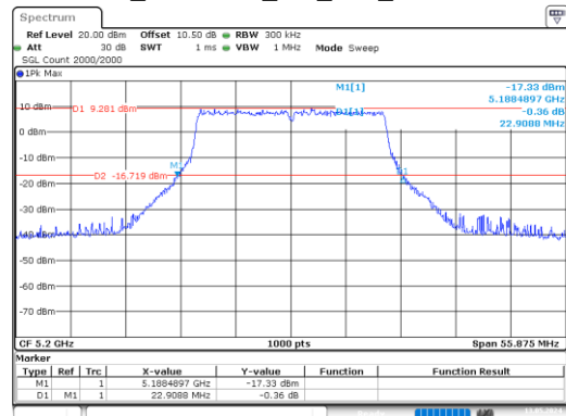
ax20_5200MHz_RU_Full_Chain 0
