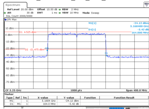
ax160_5250MHz_RU_Full_Chain 0
