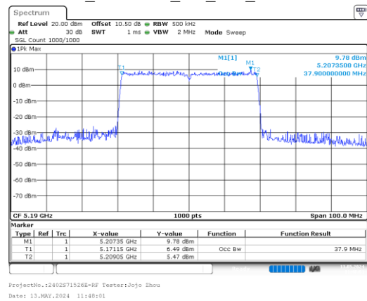
ax40_5190MHz_RU_Full_Chain 0
