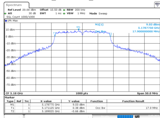
n20_5180MHz_Chain 0
