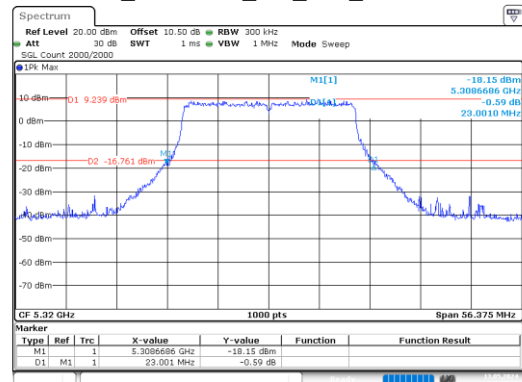
ax20_5320MHz_RU_Full_Chain 0
