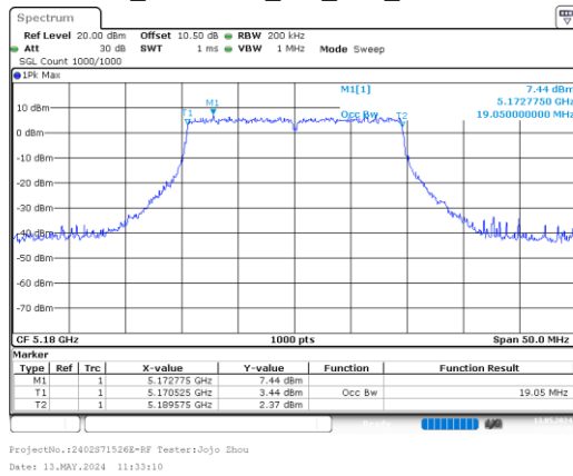
ax20_5180MHz_RU_Full_Chain 0
