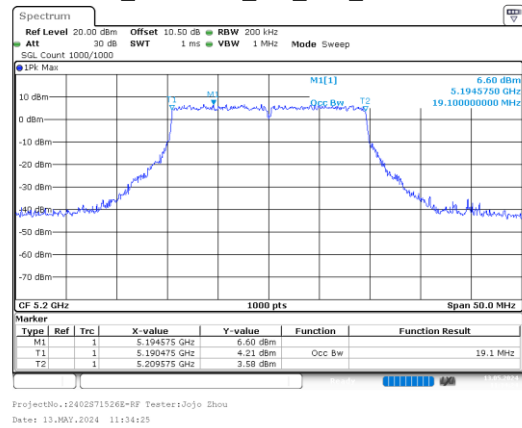
ax20_5200MHz_RU_Full_Chain 0
