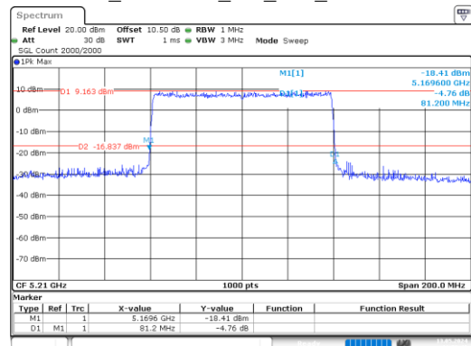
ax80_5210MHz_RU_Full_Chain 0
