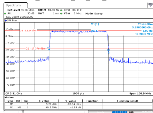
ax40_5310MHz_RU_Full_Chain 0
