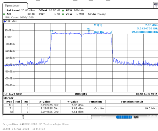
ax20_5240MHz_RU_Full_Chain 0
