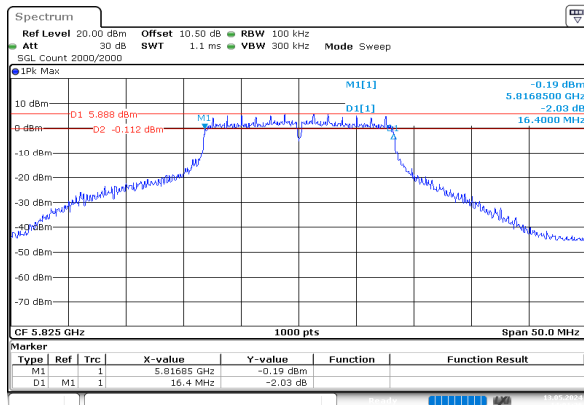
a_5825MHz_Chain 0
