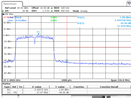
n40_2452MHz_Chain 0
