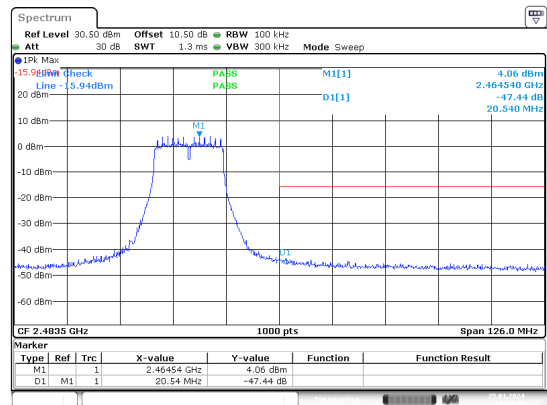
g_2462MHz_Chain 1
