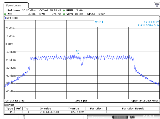
g_2412MHz_Chain 1
