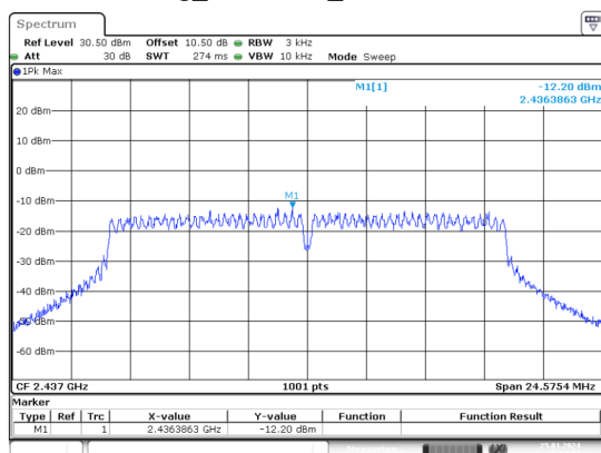
g_2437MHz_Chain 0
