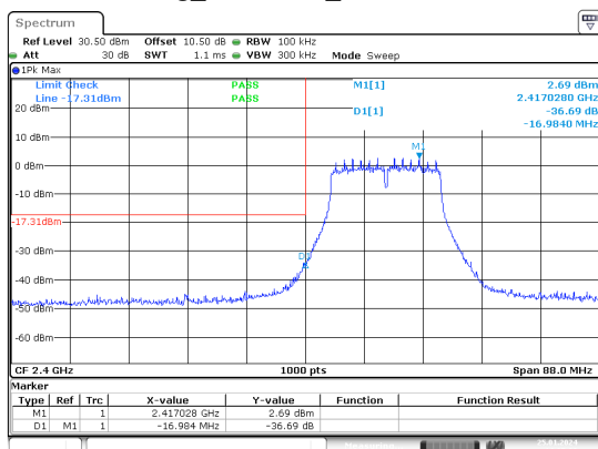
g_2412MHz_Chain 0
