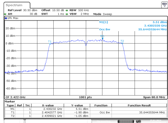
n40_2422MHz_Chain 0
