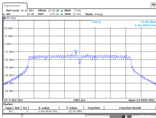
g_2462MHz_Chain 0
