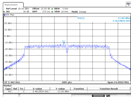
g_2462MHz_Chain 1
