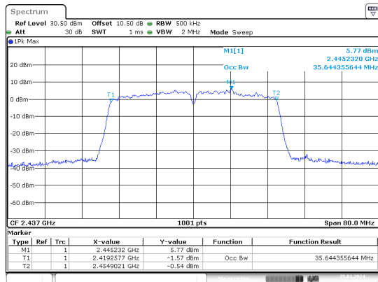
n40_2437MHz_Chain 0
