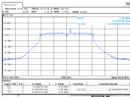
g_2437MHz_Chain 0
