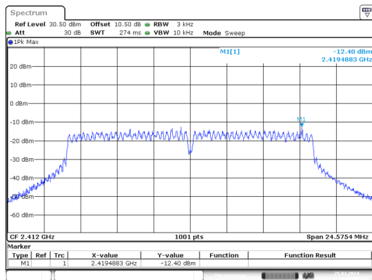
g_2412MHz_Chain 0
