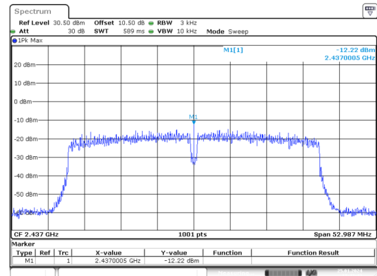
n40_2437MHz_Chain 1
