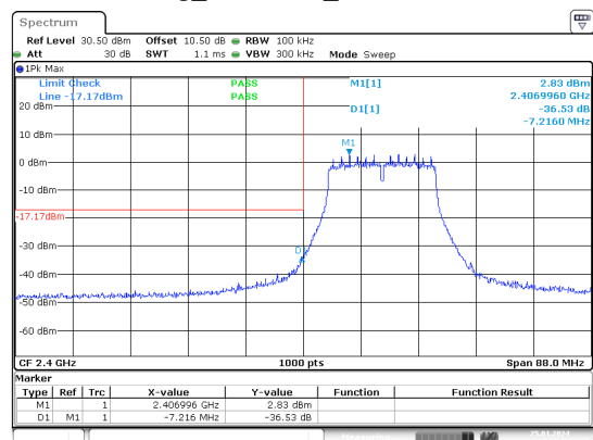
g_2412MHz_Chain 1
