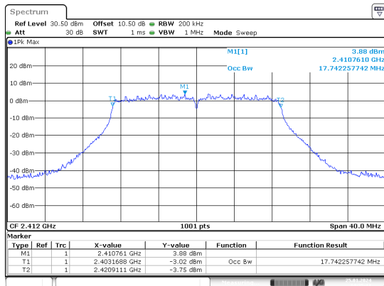
n20_2412MHz_Chain 0
