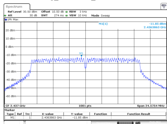
g_2437MHz_Chain 1
