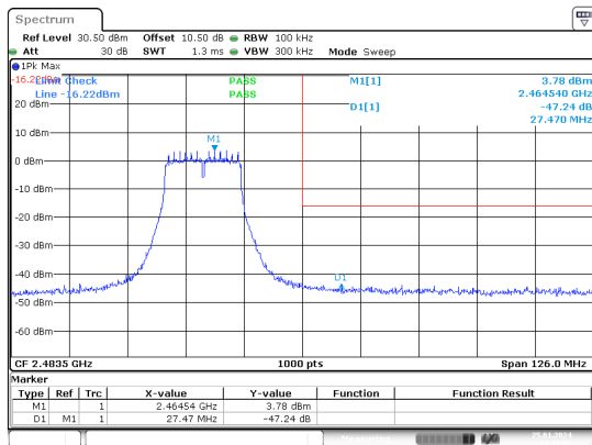
g_2462MHz_Chain 0
