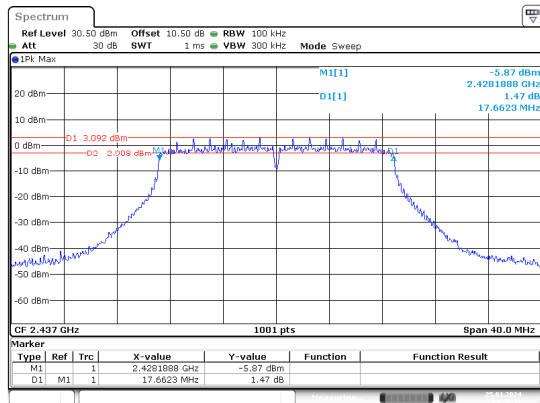
n20_2437MHz_Chain 0
