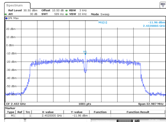
n40_2452MHz_Chain 1
