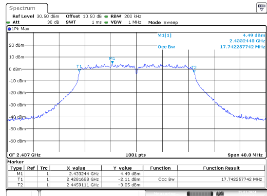
n20_2437MHz_Chain 0
