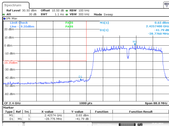
n40_2422MHz_Chain 0
