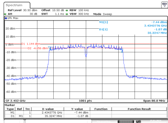
n40_2452MHz_Chain 0
