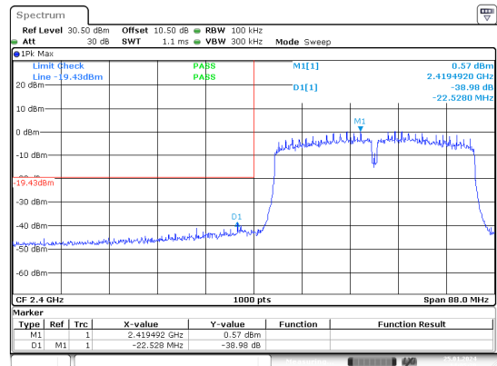
n40_2422MHz_Chain 1
