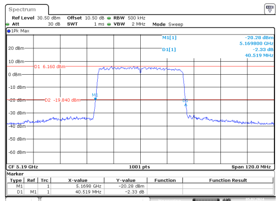
ax40_5190MHz_RU_FULL_Chain 0
