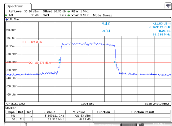
ax80_5210MHz_RU_FULL_Chain 0
