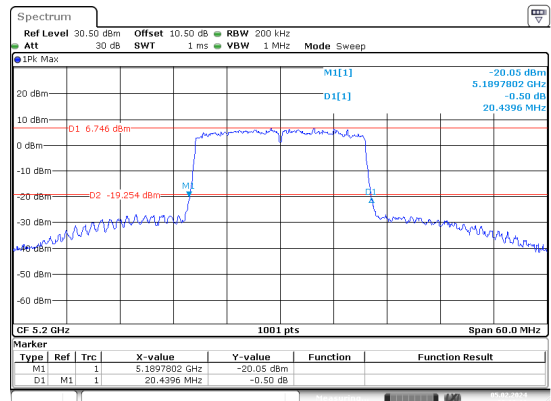
ax20_5200MHz_RU_FULL_Chain 0
