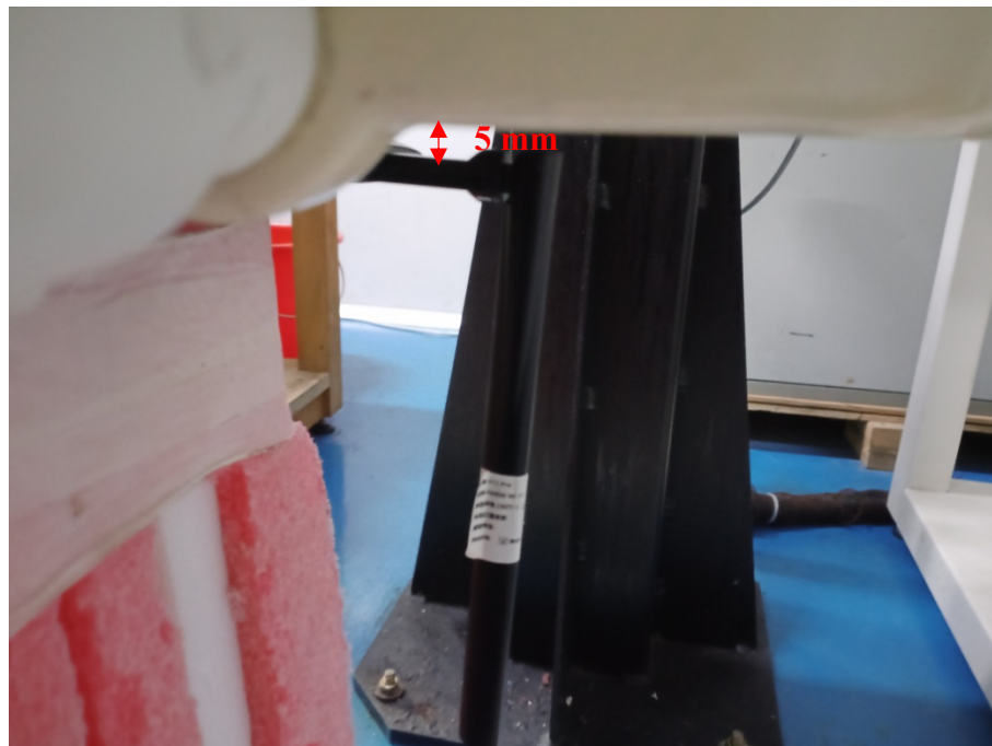
Horizontal-Up With Antenna Fold Setup Photo(5mm)
