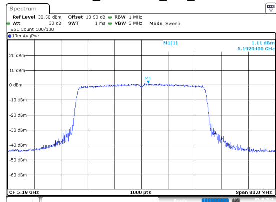
ax40_5190MHz_RU_Full
