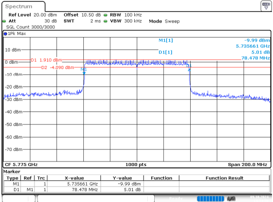
ax80_5775MHz_RU_Full
