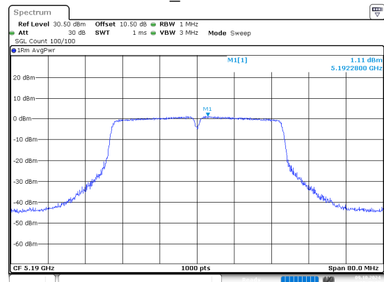
ac40_5190MHz
