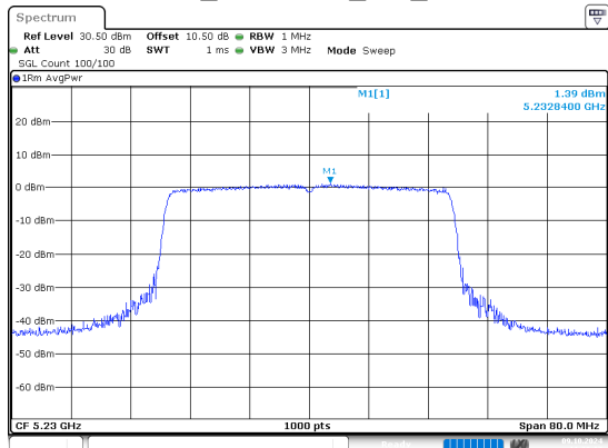
ax40_5230MHz_RU_Full
