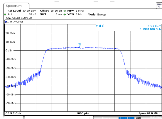
ax20_5200MHz_RU_Full
