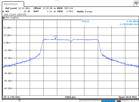
a_5745MHz
