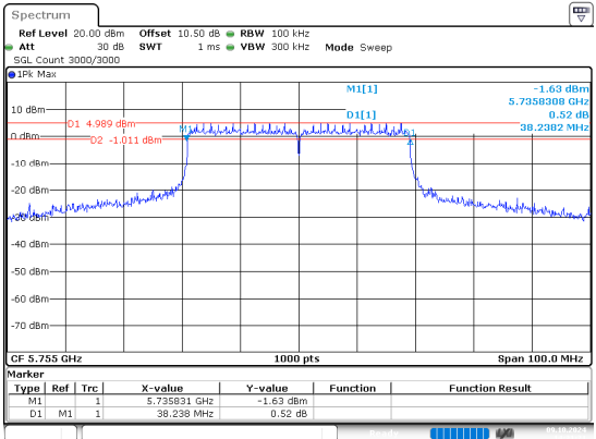
ax40_5755MHz_RU_Full
