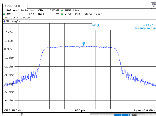
ax20_5180MHz_RU_Full
