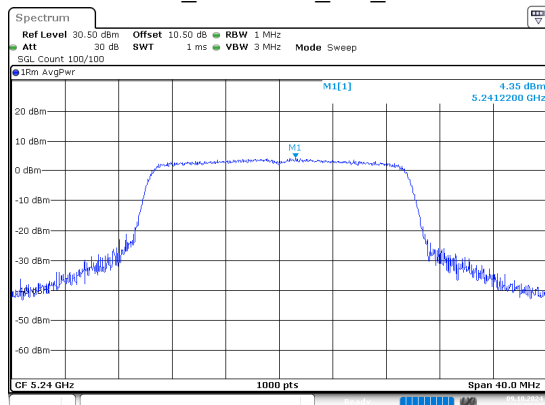
ax20_5240MHz_RU_Full
