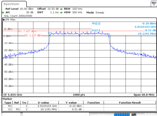
ax20_5825MHz_RU_Full
