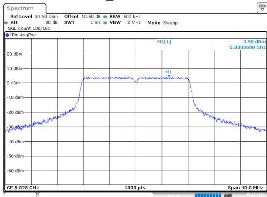
a_5825MHz
