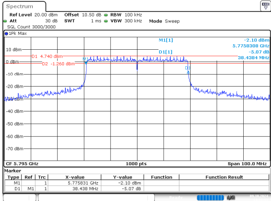
ax40_5795MHz_RU_Full
