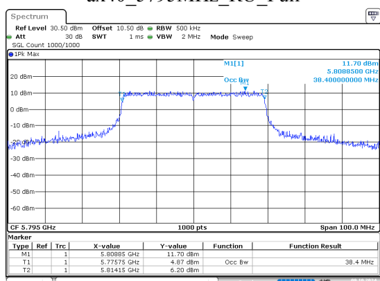
ax40_5795MHz_RU_Full
