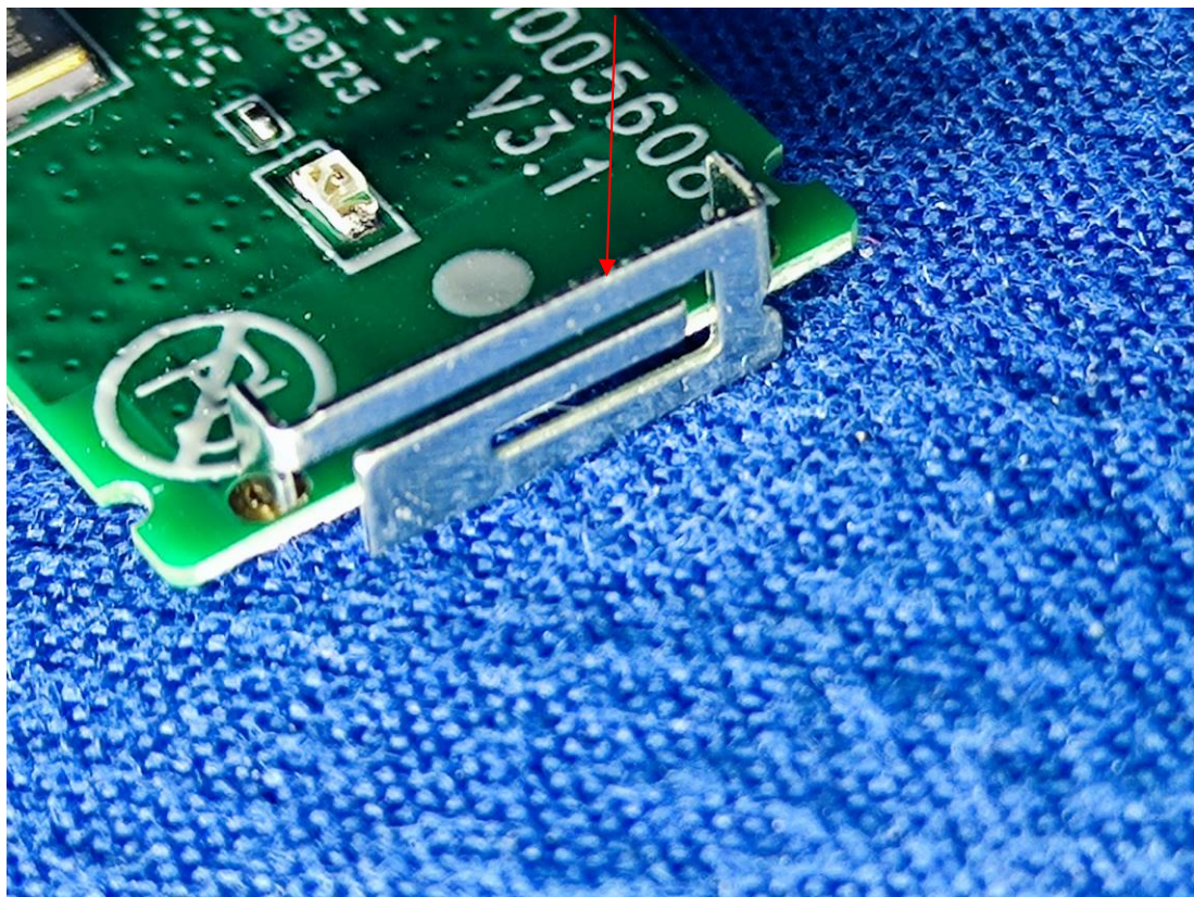
2.4G Wifi&5G Wifi Antenna
