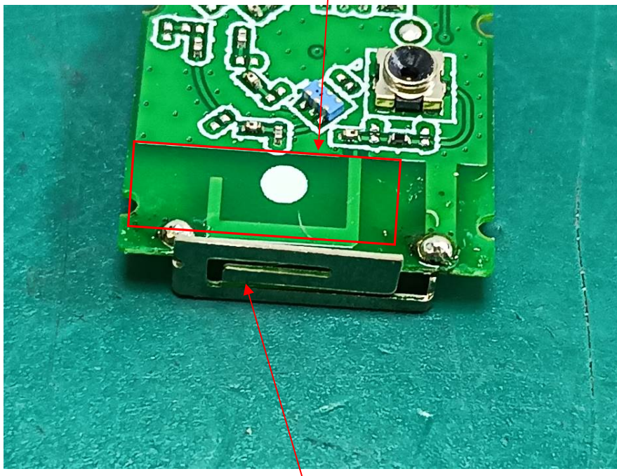
BT&BLE&2.4G WIFI ANT
