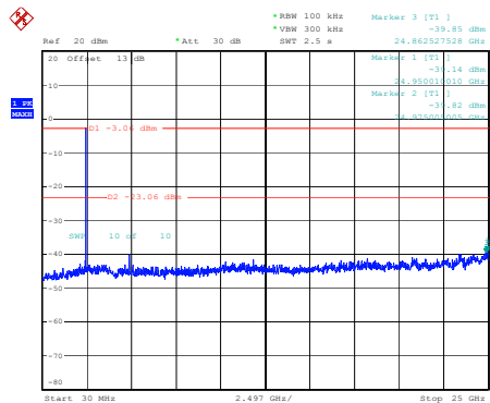
BLE_2M_Middle_Channel
