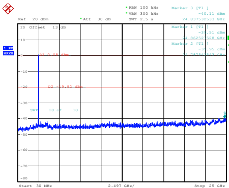
BLE_2M_High_Channel
