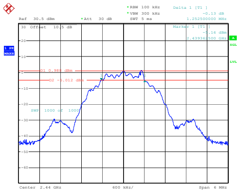
BLE_2M_Middle_Channel
