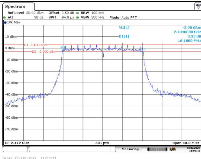
6dB Emission Bandwidth
