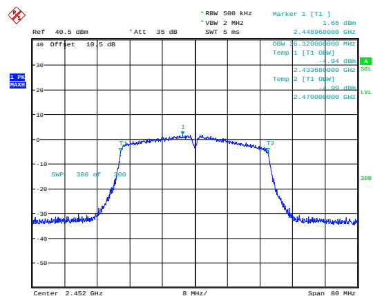
802.11n40_2452MHz_Chain 0
