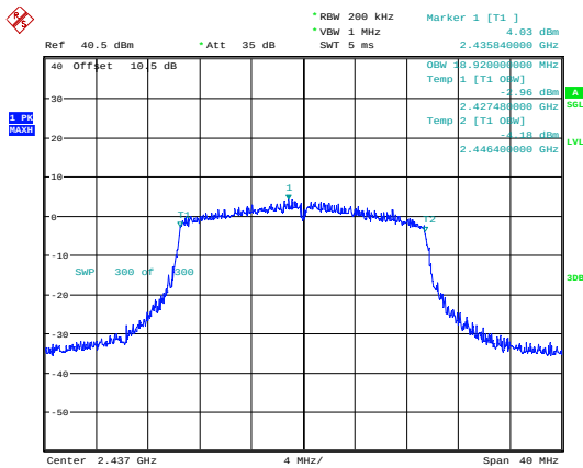
802.11ax20_2437MHz_RU_Full_Chain 0
