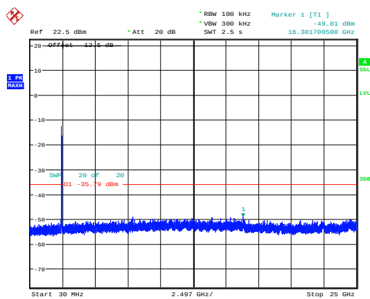
802.11ax40_2422MHz_RU_Full_Chain 1
