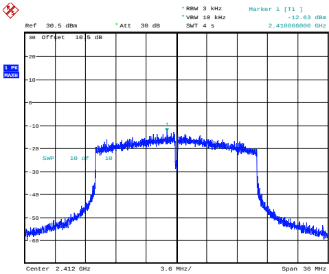
802.11ax20_2412MHz_RU_Full_Chain 0
