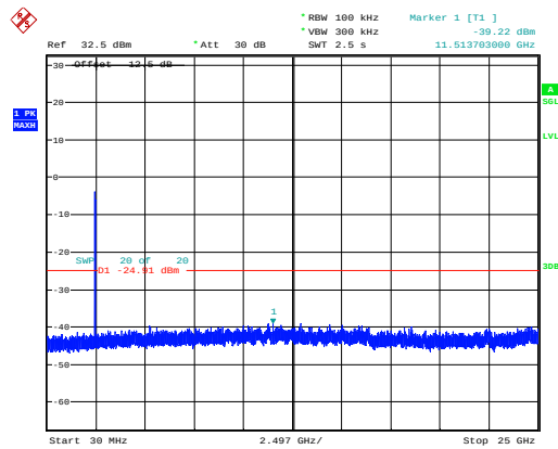
802.11g_2462MHz_Chain 1
