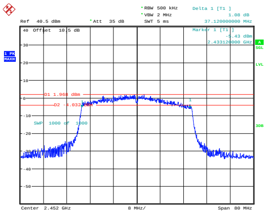
802.11ax40_2452MHz_RU_Full_Chain 0
