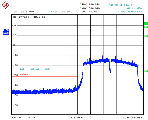
802.11n40_2422MHz_Chain 1
