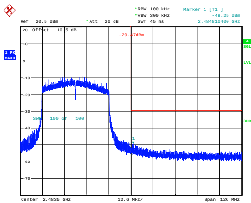
802.11ax40_2452MHz_RU_Full_Chain 0
