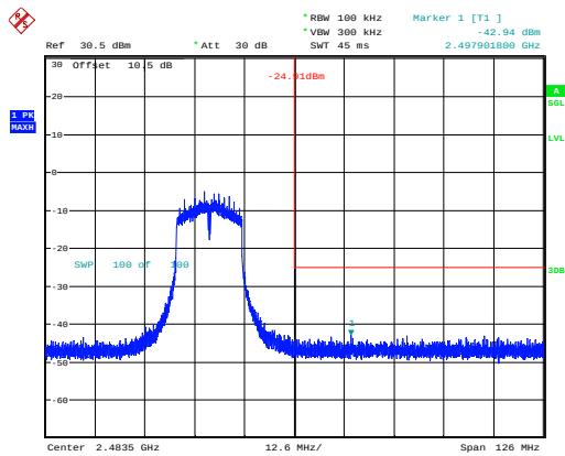
802.11g_2462MHz_Chain 1
