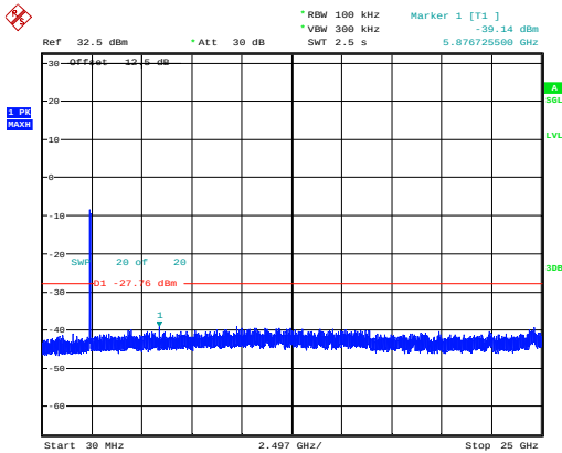
802.11n40_2422MHz_Chain 0
