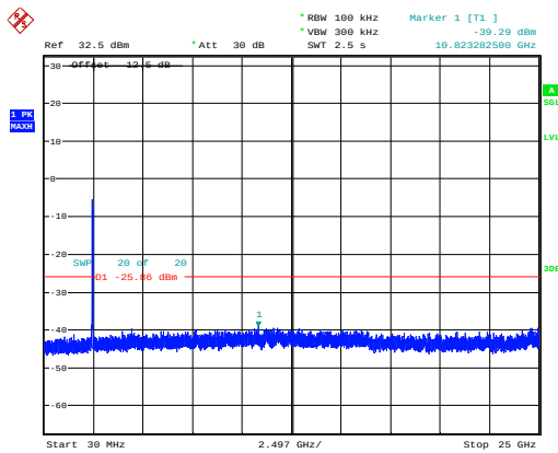
802.11n40_2452MHz_Chain 0
