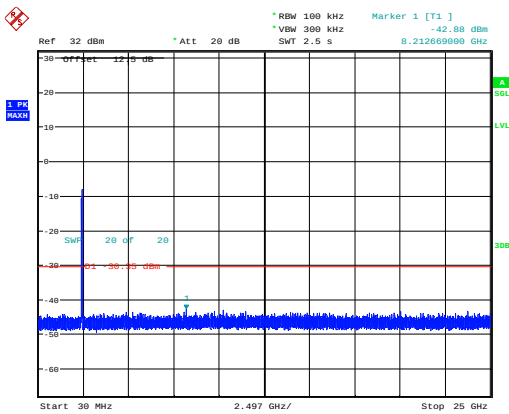
802.11n40_2437MHz_Chain 1
