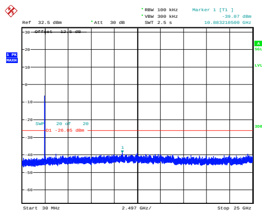
802.11ax20_2462MHz_RU_Full_Chain 1
