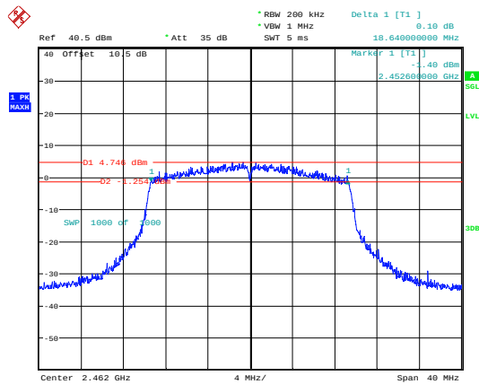
802.11ax20_2462MHz_RU_Full_Chain 0
