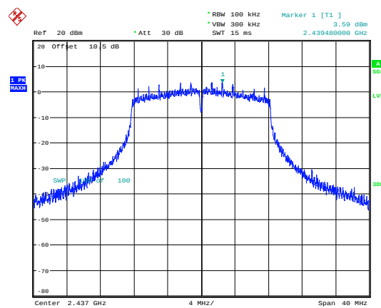
802.11g_2437MHz_Chain 0
