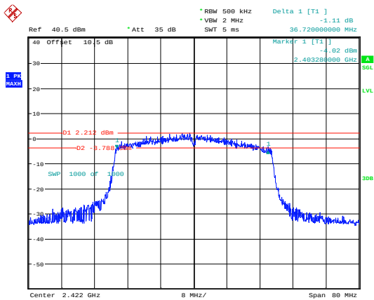
802.11ax40_2422MHz_RU_Full_Chain 0
