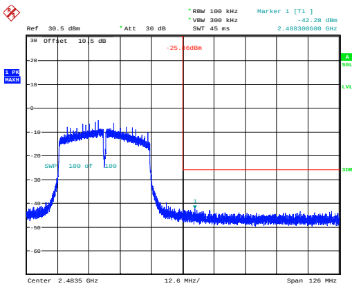
802.11n40_2452MHz_Chain 0
