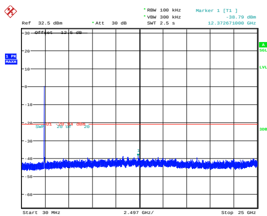
802.11ax20_2412MHz_RU_Full_Chain 0
