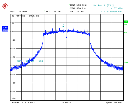
802.11g_2412MHz_Chain 0
