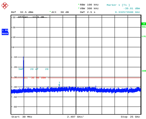
802.11n40_2422MHz_Chain 1
