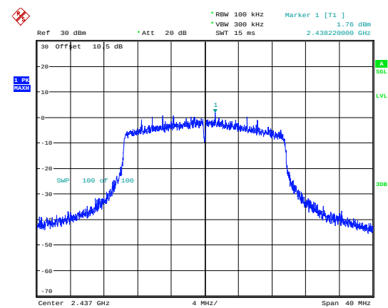
802.11ax20_2437MHz_RU_Full_Chain 0
