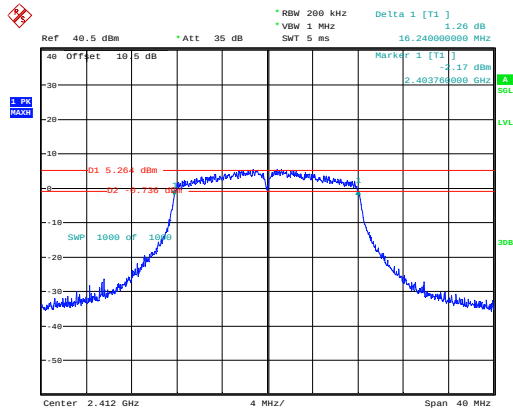
802.11g_2412MHz_Chain 0
