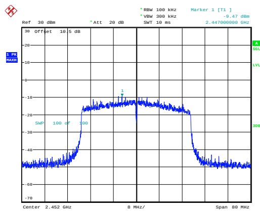
802.11ax40_2452MHz_RU_Full_Chain 0
