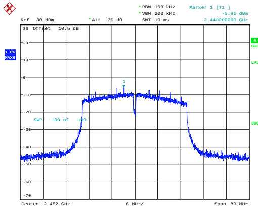
802.11n40_2452MHz_Chain 0
