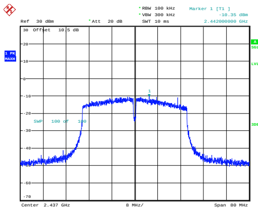
802.11n40_2437MHz_Chain 1
