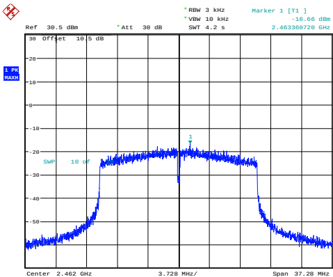
802.11ax20_2462MHz_RU_Full_Chain 1
