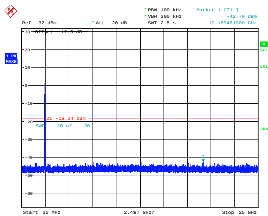
802.11ax20_2437MHz_RU_Full_Chain 0
