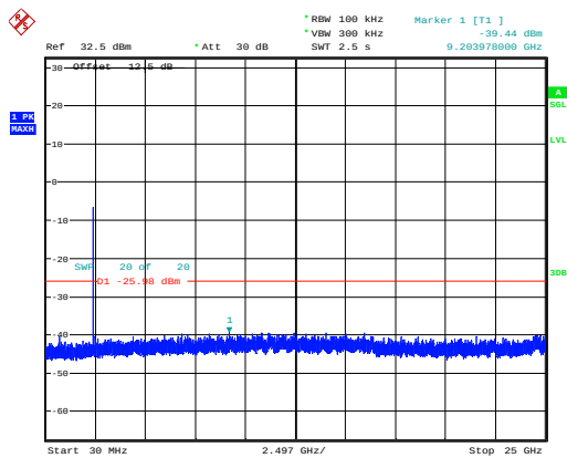
802.11ax20_2412MHz_RU_Full_Chain 1
