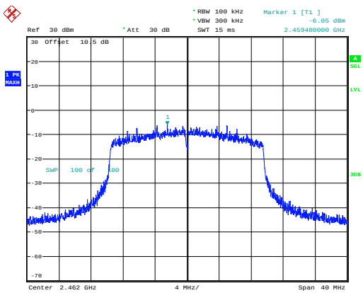
802.11ax20_2462MHz_RU_Full_Chain 1
