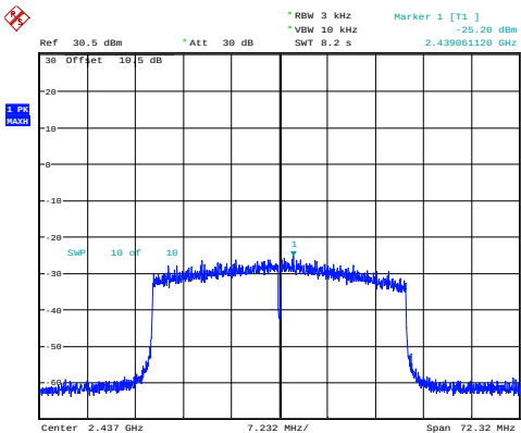
802.11ax40_2437MHz_RU_Full_Chain 1
