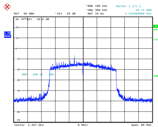
802.11ax40_2437MHz_RU_Full_Chain 1
