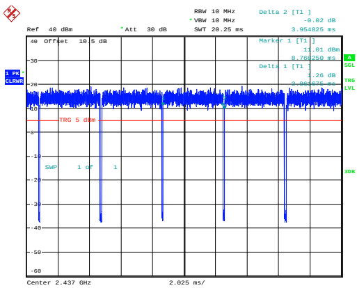
802.11ax40_2437MHz_RU_Full_Chain 0
