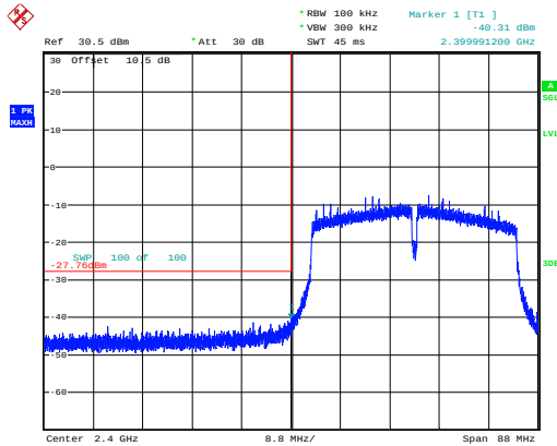
802.11n40_2422MHz_Chain 0
