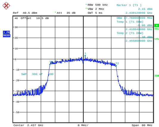
802.11ax40_2437MHz_RU_Full_Chain 0
