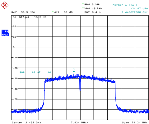
802.11ax40_2452MHz_RU_Full_Chain 1
