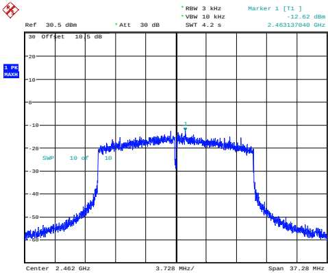
802.11ax20_2462MHz_RU_Full_Chain 0
