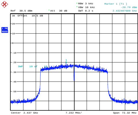
802.11ax40_2437MHz_RU_Full_Chain 0
