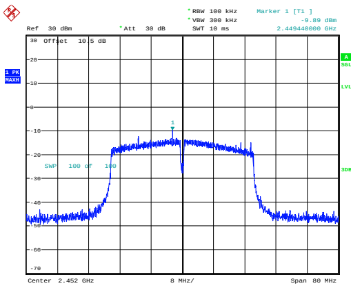
802.11n40_2452MHz_Chain 1
