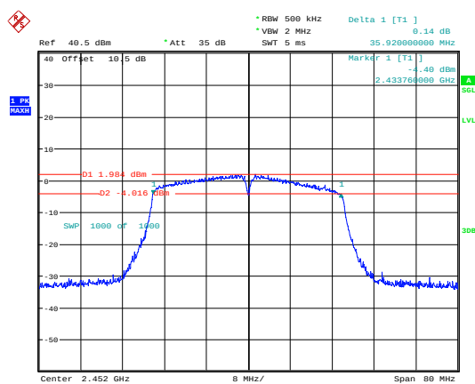
802.11n40_2452MHz_Chain 0
