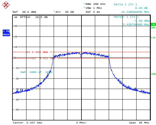
802.11g_2437MHz_Chain 0
