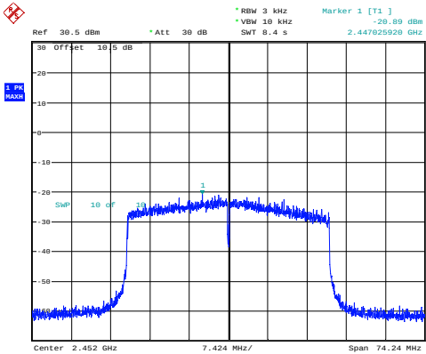
802.11ax40_2452MHz_RU_Full_Chain 0
