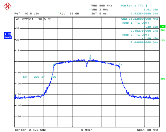
802.11n40_2422MHz_Chain 0
