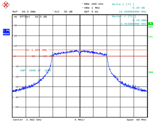
802.11g_2462MHz_Chain 0
