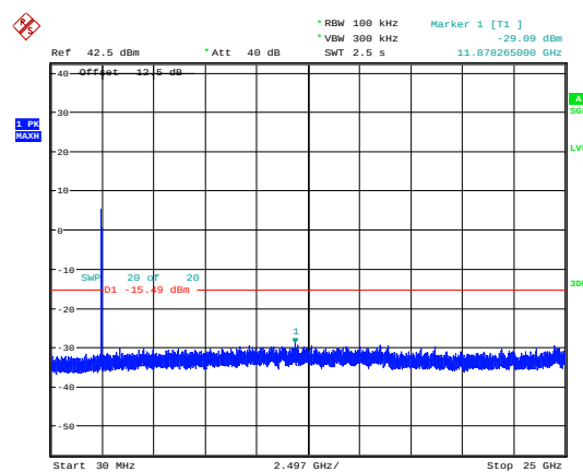
802.11g_2462MHz_Chain 0
