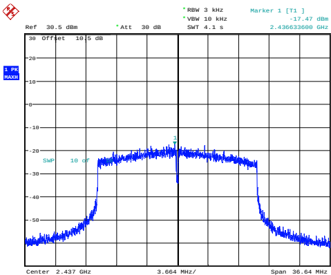
802.11ax20_2437MHz_RU_Full_Chain 1
