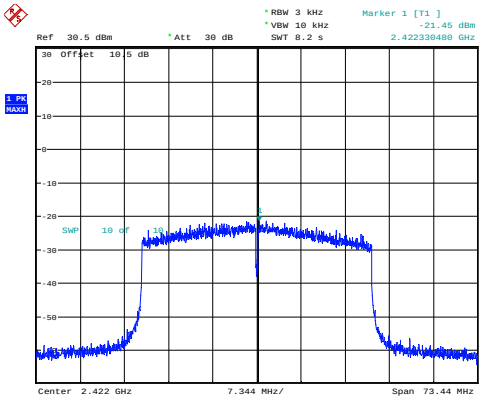
802.11ax40_2422MHz_RU_Full_Chain 0
