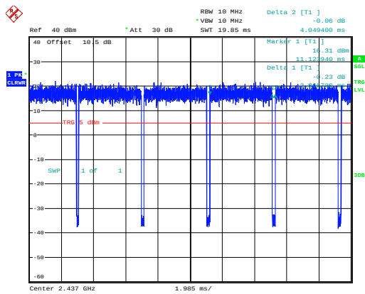
802.11ax20_2437MHz_RU_Full_Chain 0
