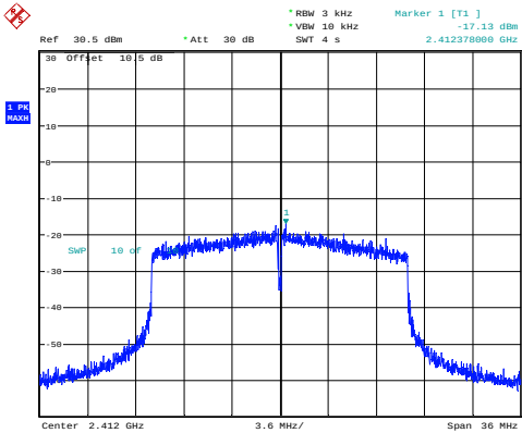
802.11ax20_2412MHz_RU_Full_Chain 1
