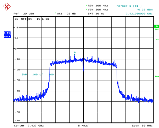
802.11ax40_2437MHz_RU_Full_Chain 0
