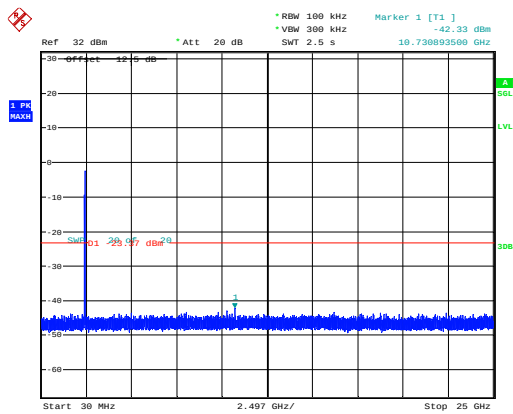
802.11ax20_2437MHz_RU_Full_Chain 1
