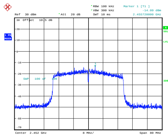
802.11ax40_2452MHz_RU_Full_Chain 1
