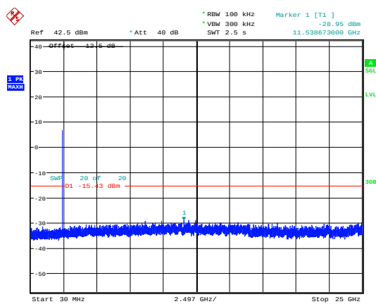
802.11g_2412MHz_Chain 0
