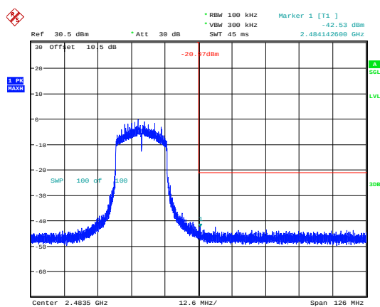
802.11ax20_2462MHz_RU_Full_Chain 0
