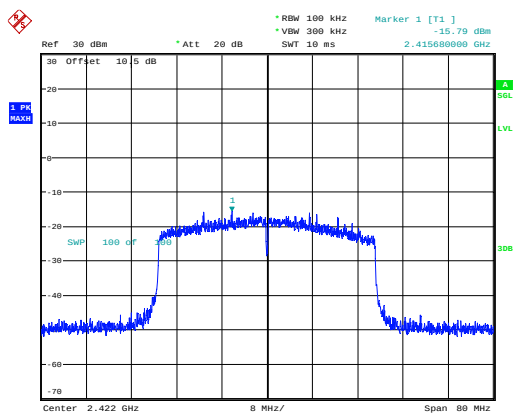
802.11ax40_2422MHz_RU_Full_Chain 1
