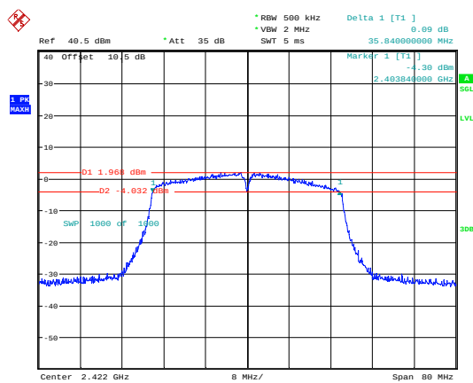
802.11n40_2422MHz_Chain 0
