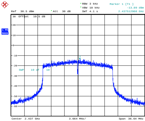
802.11ax20_2437MHz_RU_Full_Chain 0
