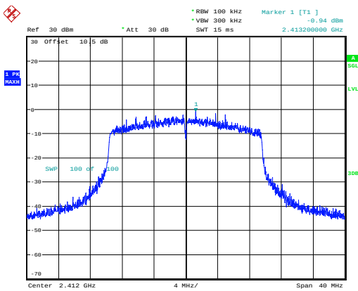
802.11ax20_2412MHz_RU_Full_Chain 0
