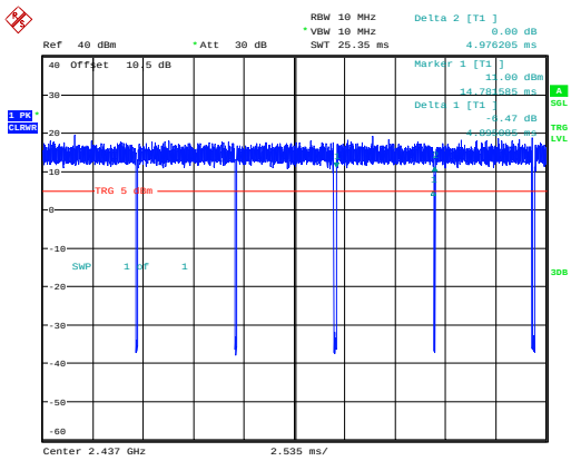
802.11n40_2437MHz_Chain 0
