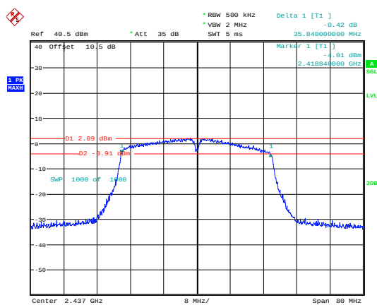
802.11n40_2437MHz_Chain 0
