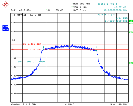
802.11ax20_2412MHz_RU_Full_Chain 0
