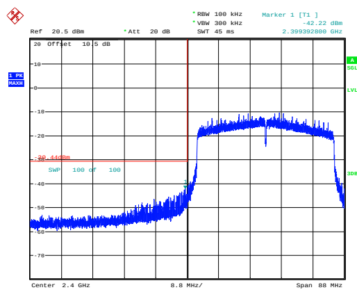
802.11ax40_2422MHz_RU_Full_Chain 0
