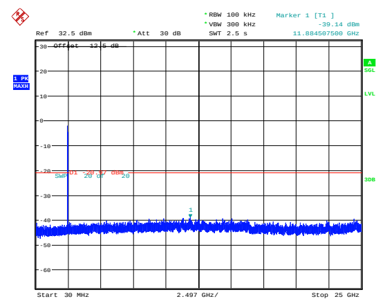
802.11ax20_2462MHz_RU_Full_Chain 0
