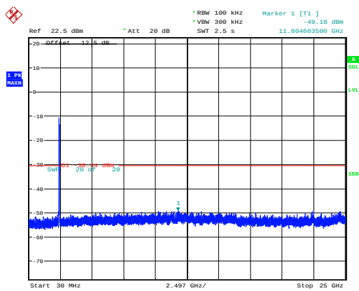
802.11ax40_2422MHz_RU_Full_Chain 0
