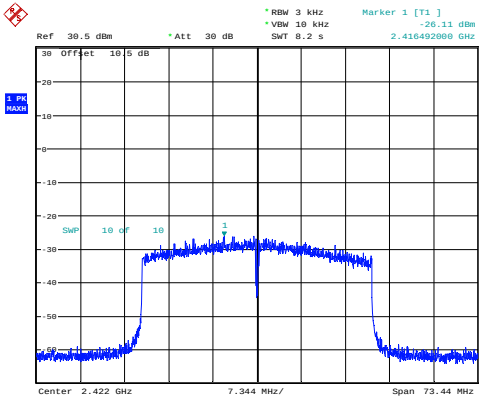
802.11ax40_2422MHz_RU_Full_Chain 1
