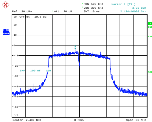
802.11n40_2437MHz_Chain 0
