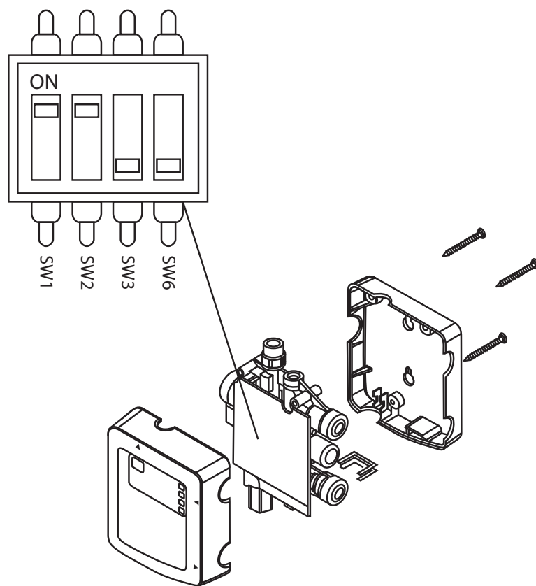
Figure 4. Dip Switches
