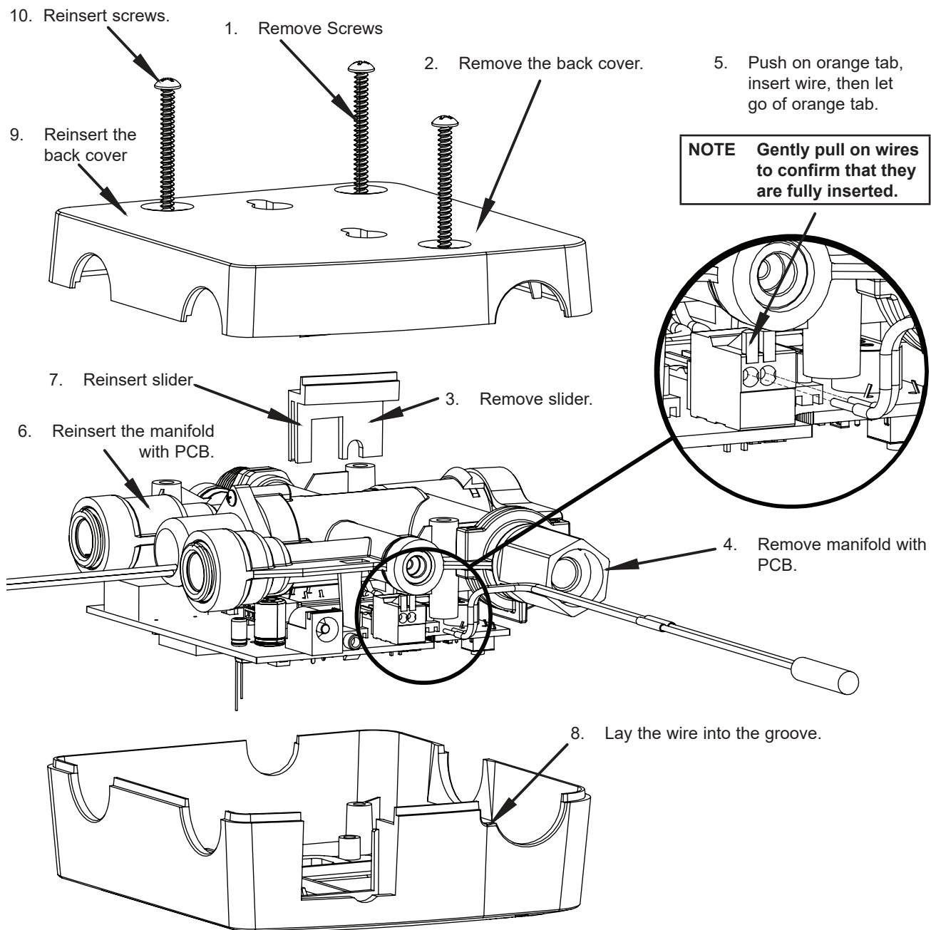
Figure 14. Flow Switch Wiring
