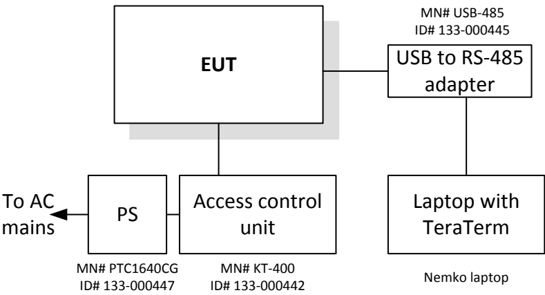
Figure 3.6-1: Setup diagram
