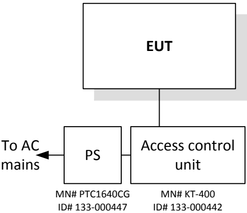
Figure 3.6-1: Setup diagram
