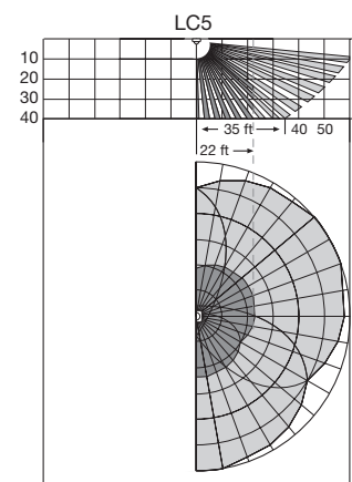
LC5 180° half moon lens cover for HBS 300
