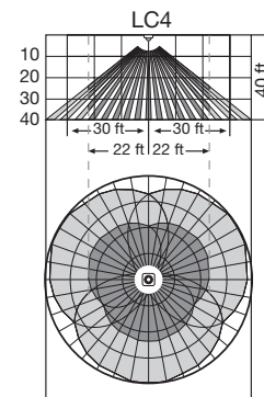
LC4 reduced range lens cover for HBS 300
