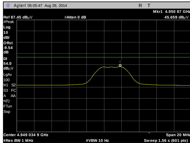
Plot 31. Radiated Spurious Emissions, High Channel, 1 MHz – 7 GHz, Average, Zoom
