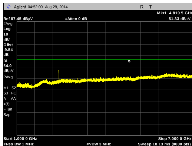
Plot 20. Radiated Spurious Emissions, Low Channel, 1 GHz – 7 GHz, Average
