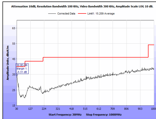
Plot 19. Radiated Spurious Emissions, Low Channel, 30 MHz – 1 GHz
