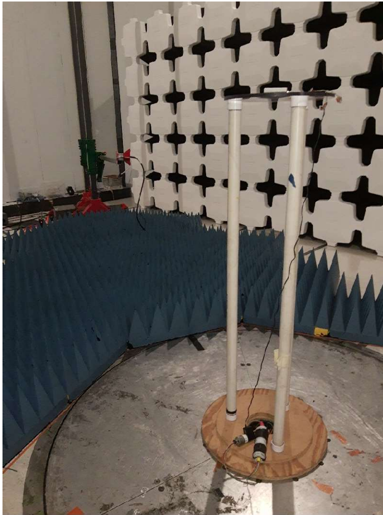
Photograph 3. Radiated Emissions, Test Setup - 1-18GHz
