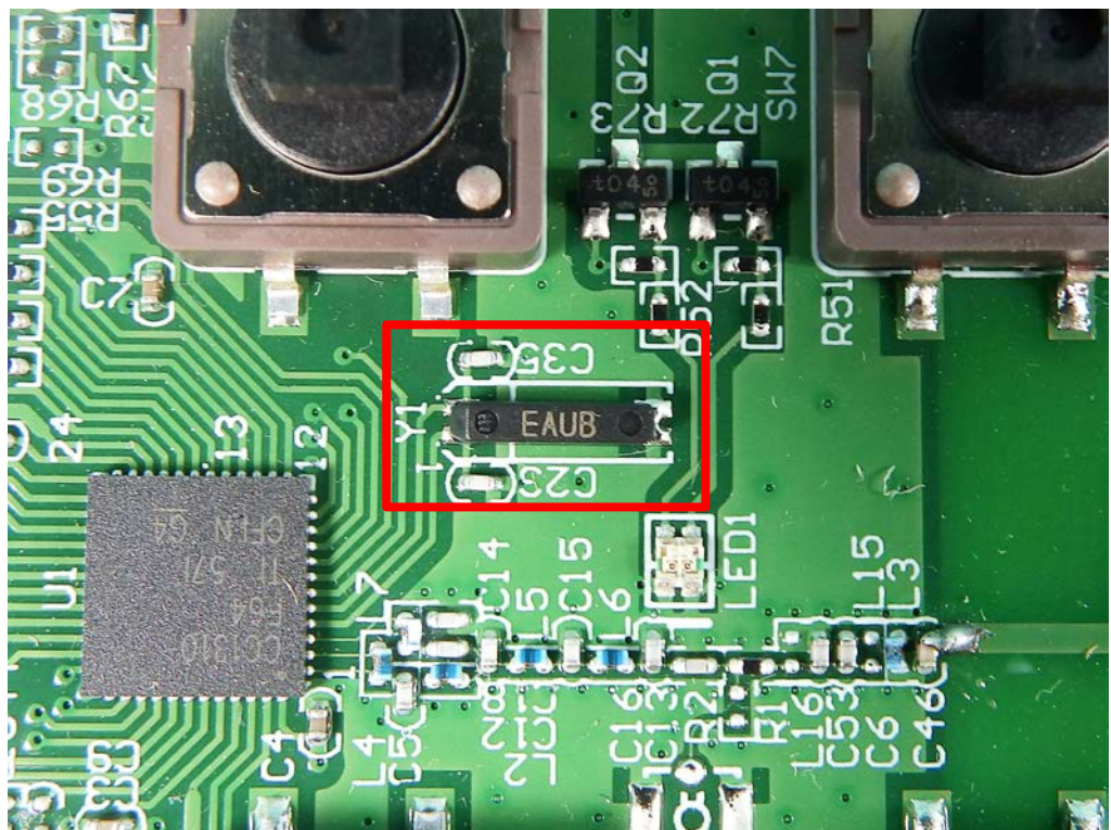
chip antenna
