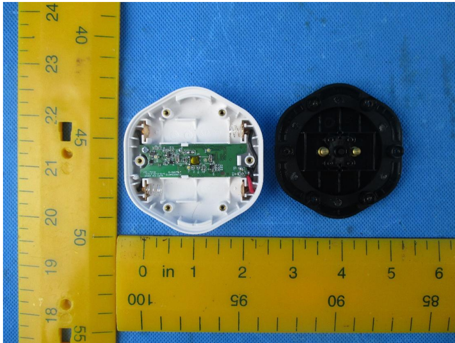
ZigBee Antenna
