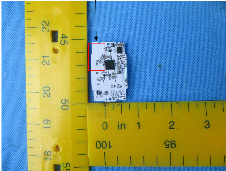
ZigBee Antenna
