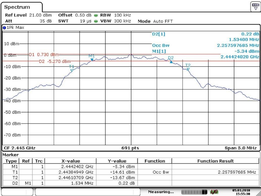
Middle channel 2445MHz
