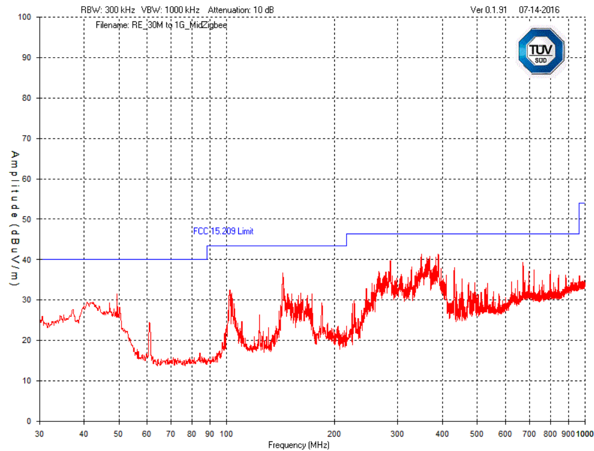
Vertical – Peak Emissions Graph – 30MHz to 1GHz (Worst case)
