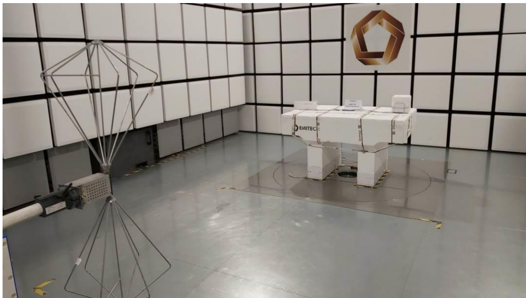
TEST SETUP PHOTO(S) - RADIATED MEASUREMENT / 30MHZ TO 200MHZ
