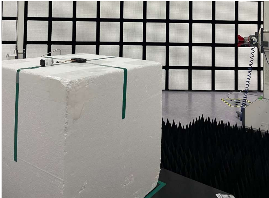
ABOVE 1 GHz REAR TEST PHOTO
