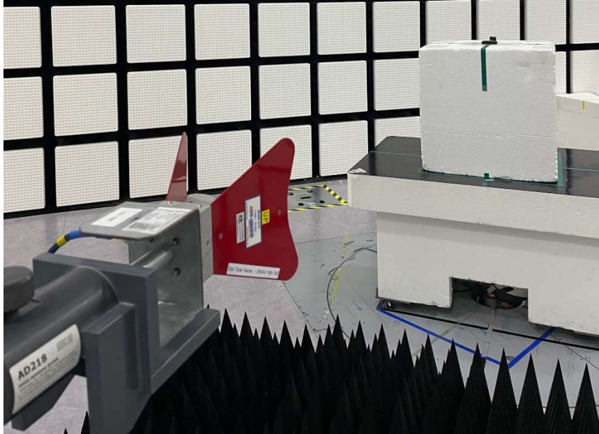
ABOVE 1 GHz FRONT TEST PHOTO
