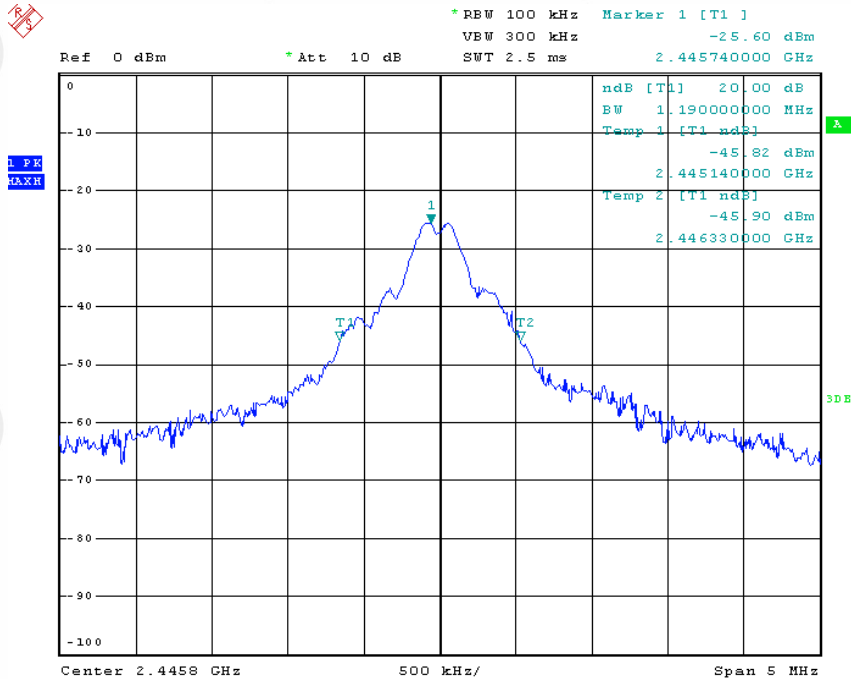
Channel low
