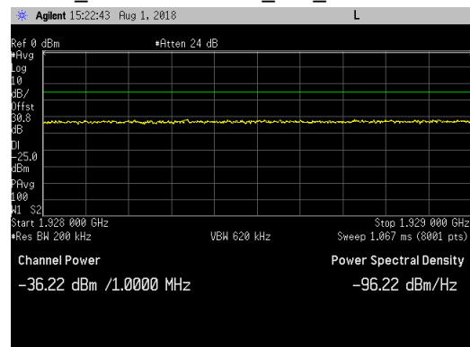
LTE20_Bottom Channel_LBE_1928 to 1929MHz
