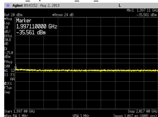
LTE20_Top Channel_UBE_1997 to 2017MHz
