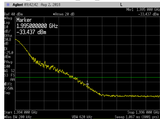
LTE20_Top Channel_UBE_1994 to 1996MHz
