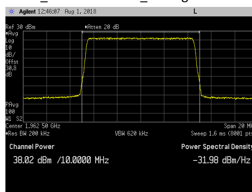
LTE10_Middle Channel_Average
