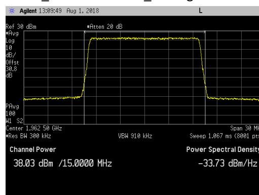
LTE15_Middle Channel_Average
