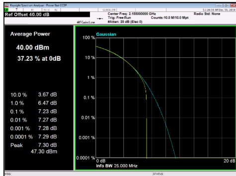
LTE5_ Middle Channel_256QAM_CCDF
