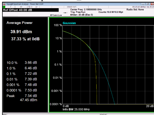
LTE10_Top Channel_CCDF
