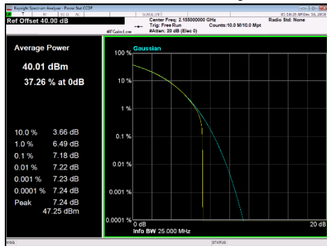
LTE5_ Middle Channel_64QAM_CCDF
