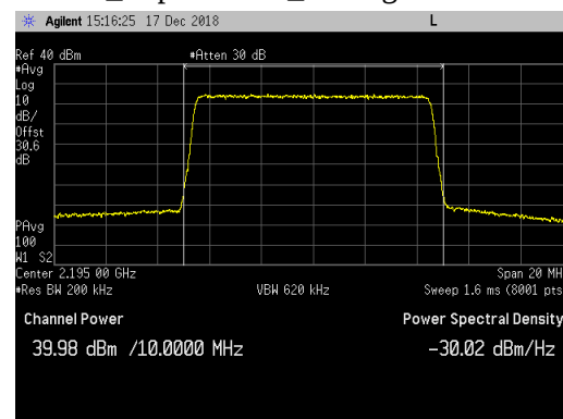
LTE10_Top Channel_Average
