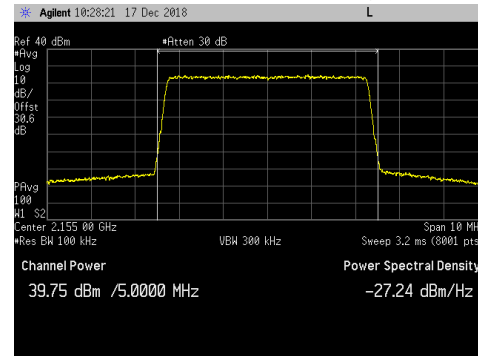
LTE5_ Middle Channel_256QAM_Average
