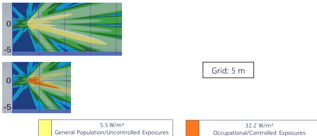
Figure 11 – Side view of the power density for the time-averaged actual maximum transmitted power of 85 W and the beam oriented in azimuth = -5° & elevation = +15° (Canada)
