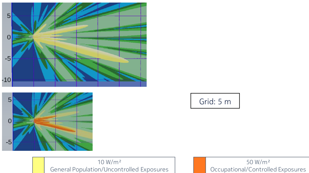
Figure 4 – Side view of the power density for the time-averaged maximum transmitted power of 339 W and the beam oriented in azimuth = -5° & elevation = +15° (EU/ICNIRP, Australia/NZ and US/related)
