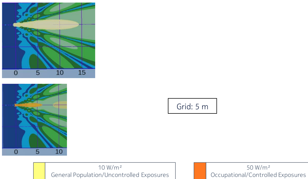
Figure 3 – Top view of the power density for the time-averaged actual maximum transmitted power of 85 W and the beam oriented in azimuth = 0° & elevation = +6° (EU/ICNIRP, Australia/NZ and US/related)
