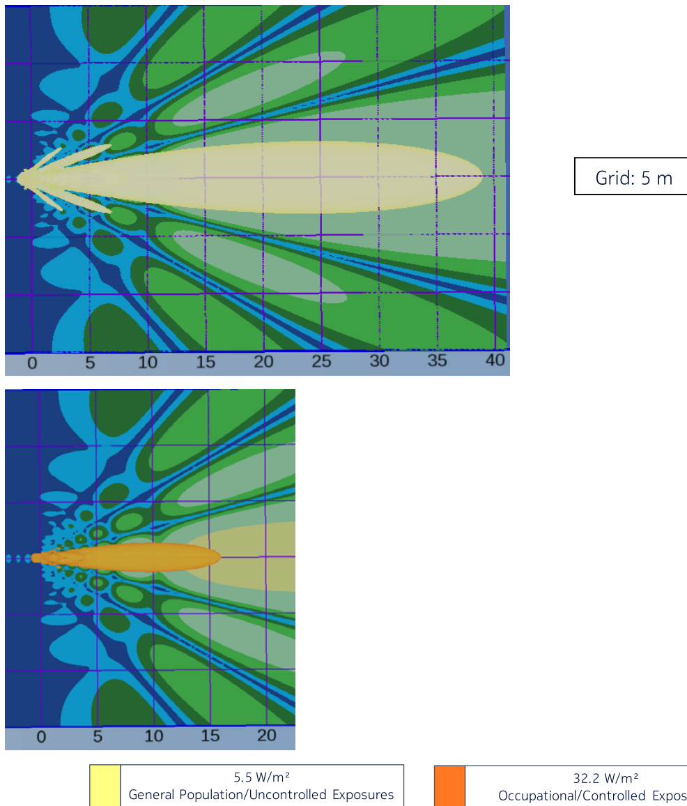
Figure 8 – Top view of the power density for the time-averaged maximum transmitted power of 339 W and the beam oriented in azimuth = 0° & elevation = +6° (Canada)
