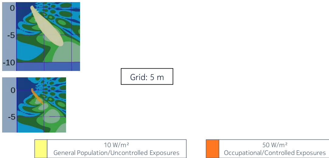
Figure 7 – Top view of the power density for the time-averaged actual maximum transmitted power of 85 W and the beam oriented in azimuth = -51° & elevation = +4° (EU/ICNIRP, Australia/NZ and US/related)
