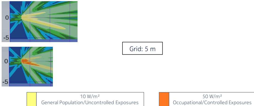
Figure 5 – Side view of the power density for the time-averaged actual maximum transmitted power of 85 W and the beam oriented in azimuth = -5° & elevation = +15° (EU/ICNIRP, Australia/NZ and US/related)
