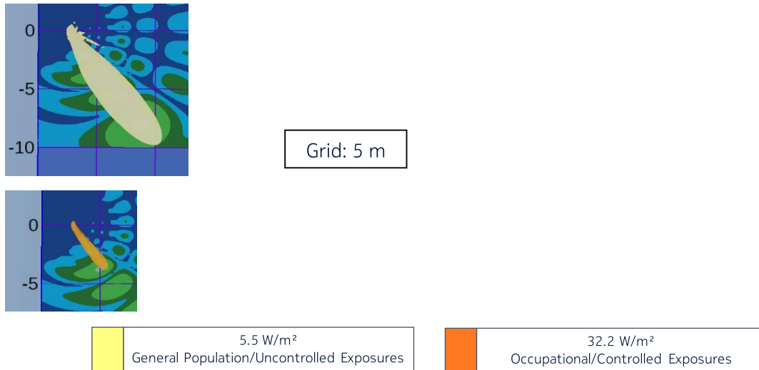
Figure 13 – Top view of the power density for the time-averaged actual maximum transmitted power of 85 W and the beam oriented in azimuth = -51° & elevation = +4° (Canada)
