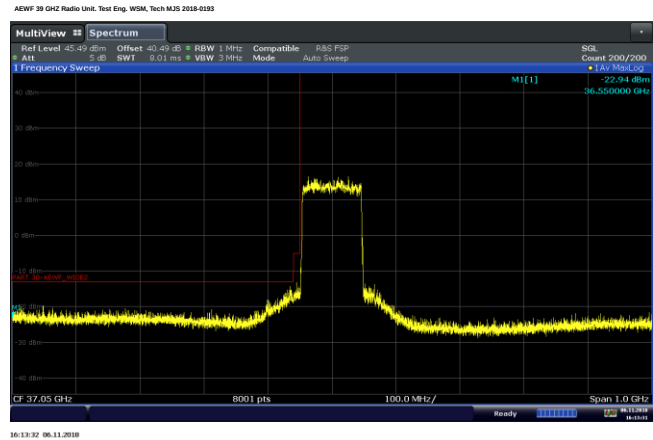
Figure 4.3.5 - Occupied Bandwidth - OOB/EoB Band Charts E
