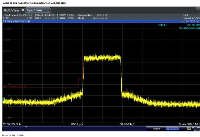
Figure 4.3.5 - Occupied Bandwidth - OOB/EoB Band Charts E
