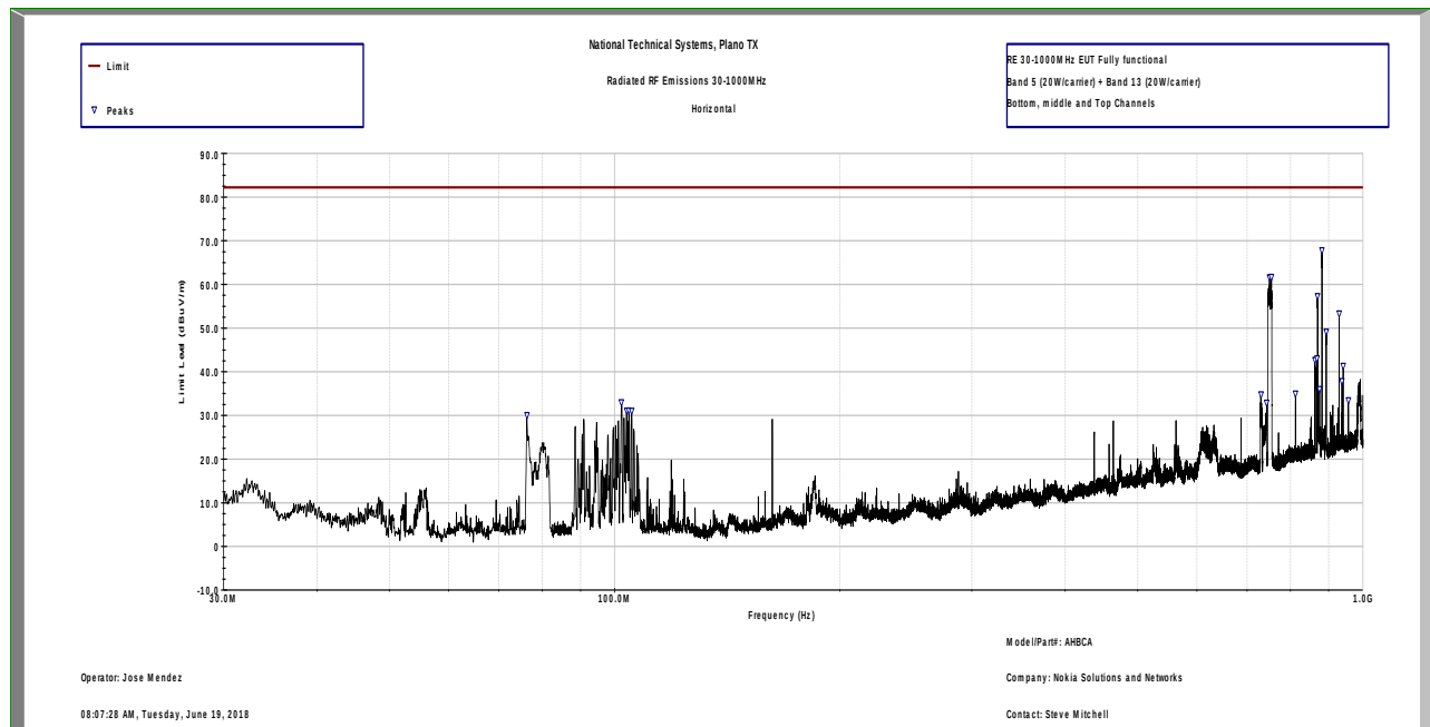
Radiated Spurious Emissions 30-1000 MHz Horizontal - Band 5 &amp; 13 Simultaneously
