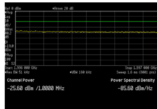
LTE5_Top Channel_UBE_1996 to 1997MHz
