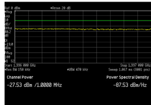
LTE15_Top Channel_UBE_1996 to 1997MHz
