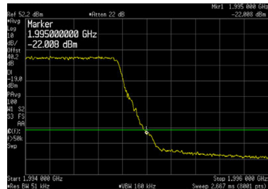
LTE5_Top Channel_UBE_1994 to 1996MHz
