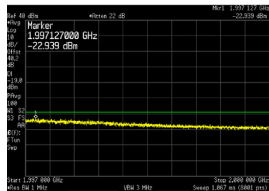
LTE5_Top Channel_UBE_1997 to 2000MHz
