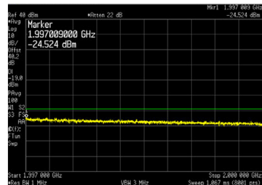
LTE10_Top Channel_UBE_1997 to 2000MHz
