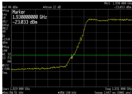
LTE5_Bottom Channel_LBE_1929 to 1931MHz
