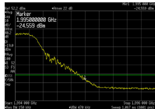
LTE15_Top Channel_UBE_1994 to 1996MHz
