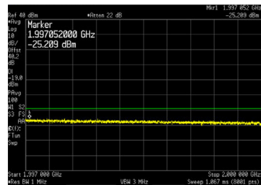
LTE15_Top Channel_UBE_1997 to 2000MHz
