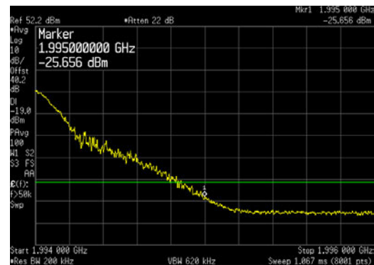
LTE20_Top Channel_UBE_1994 to 1996MHz
