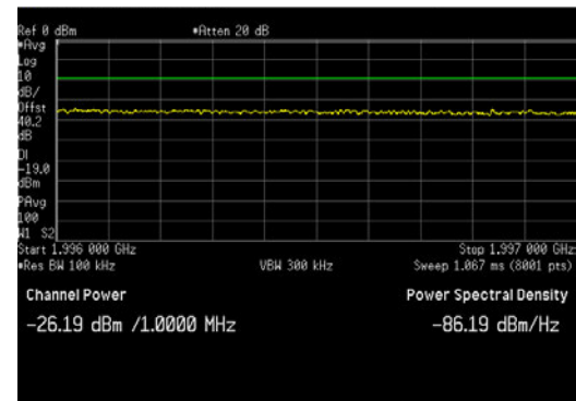
LTE10_Top Channel_UBE_1996 to 1997MHz
