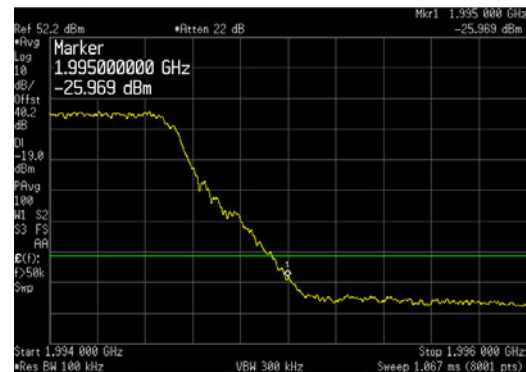
LTE10_Top Channel_UBE_1994 to 1996MHz
