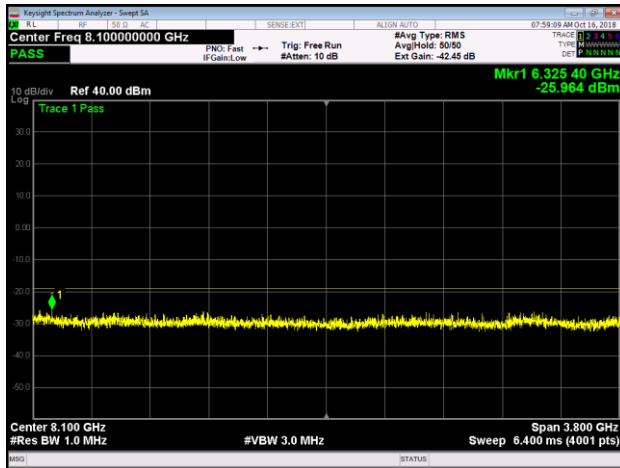
Band 66, LTE10, T, Upper, 6200MHz-10GHz
