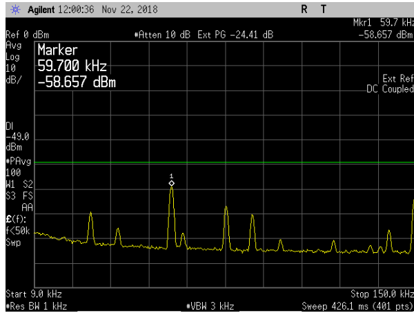
LTE15 Bottom+NB IoT GB (Upper) 9-150KHz
