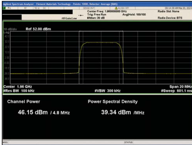
3G WCDMA PCS Band II 64QAM Modulation Mid Channel, 1960.0 MHz Port 1
