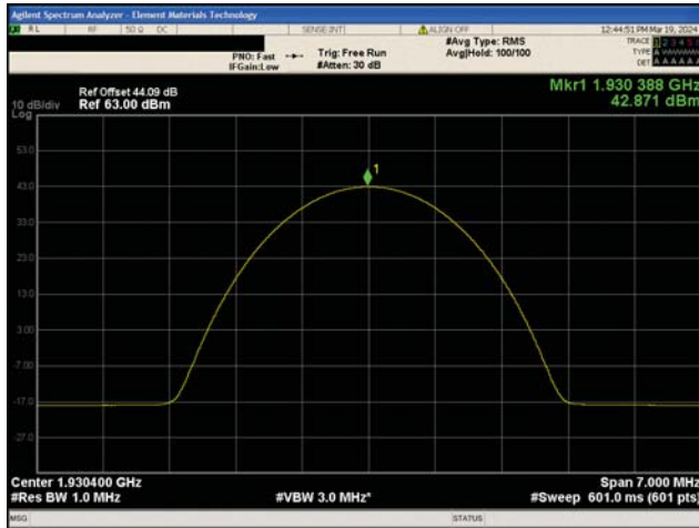
2G GSM/EDGE PCS Band 2 Test Case 3 GMSK Modulation Low Channel +1, 1930.4 MHz
