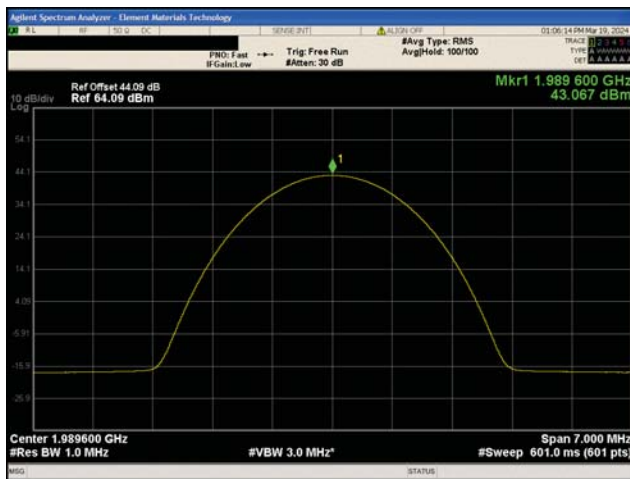
2G GSM/EDGE PCS Band 2 Test Case 3 8PSK Modulation High Channel -1, 1989.6 MHz
