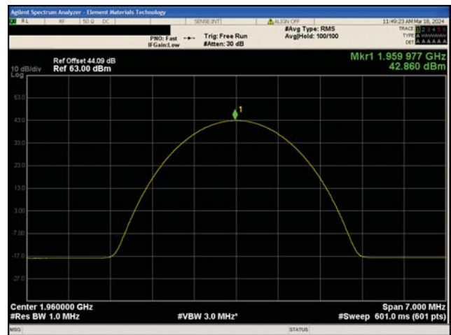
2G GSM/EDGE Band 2 GMSK Modulation Mid Channel, 1960.0 MHz Port 4
