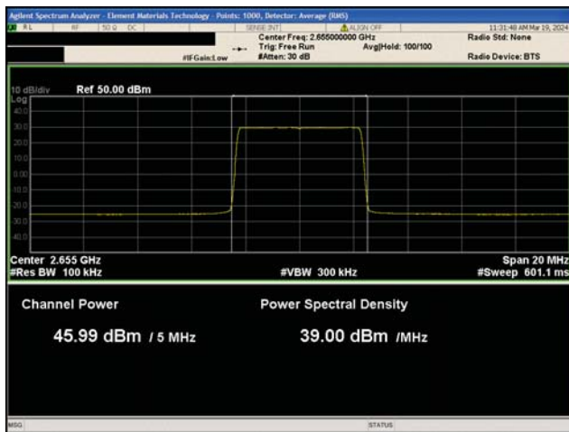
2G GSM/EDGE PCS Band 2 Test Case 2 LTE5 QPSK Modulation Mid Channel, 2655.0 MHz
