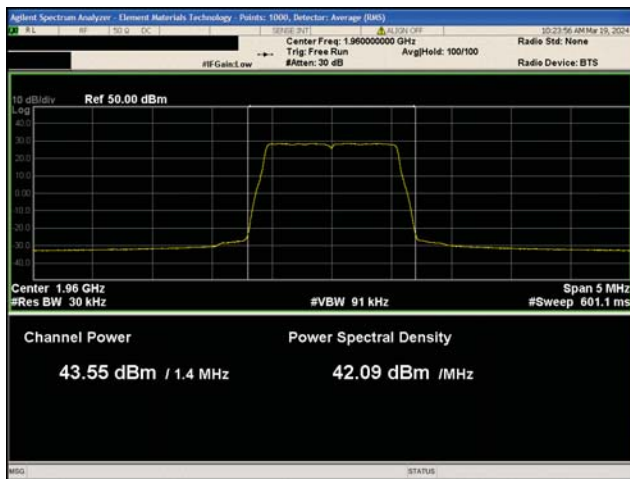
2G GSM/EDGE PCS Band 2 Test Case 1 LTE1.4 QPSK Modulation Mid Channel, 1960.0 MHz
