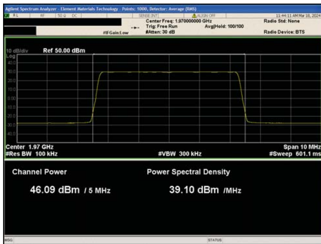
2G GSM/EDGE Band 2 LTE5 QPSK Modulation 1970.0 MHz Port 3
