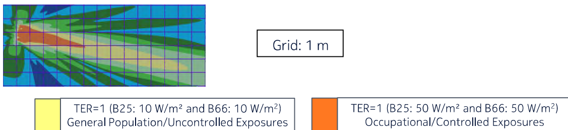
Figure 5 - Top view of the power density for the actual maximum transmitted power of 339 W (corresponding to the actual EIRP threshold of 73.42 dBm) and the beam oriented in azimuth = 0° & elevation = +12° (US/related)
