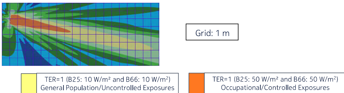
Figure 4 – Side view of the power density for the time-averaged maximum transmitted power of 678 W (corresponding to the time-averaged maximum EIRP of 76.42 dBm in the boresight direction) and the beam oriented in azimuth = 0° & elevation = +12° (US/related)
