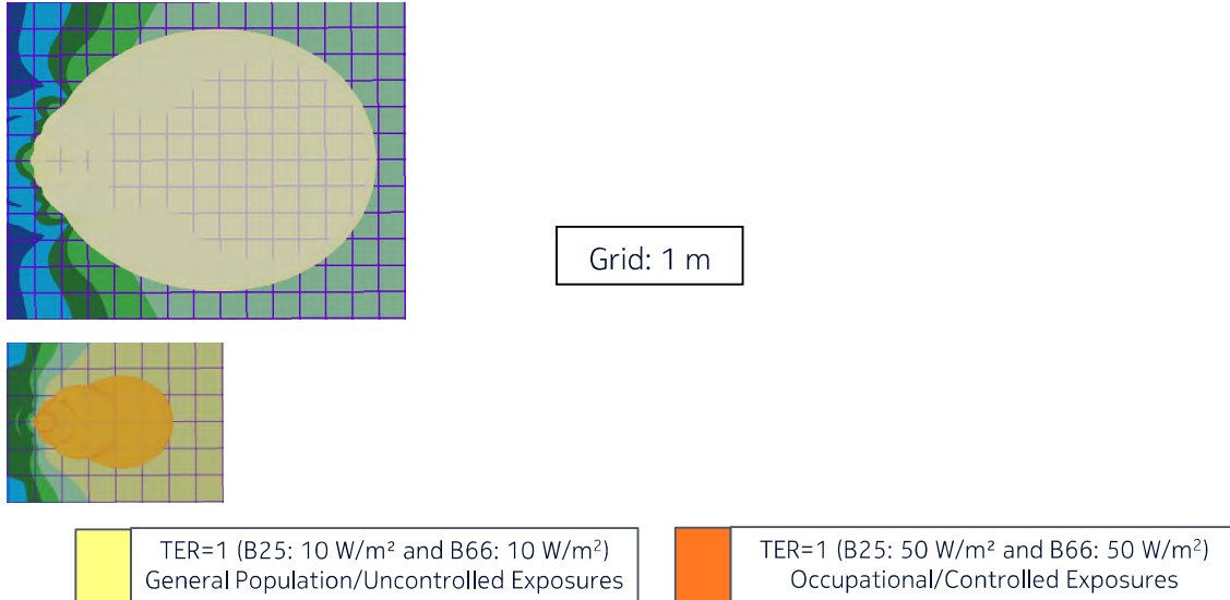
Figure 3 - Top view of the power density for the actual maximum transmitted power of 339 W (corresponding to the actual EIRP threshold of 73.42 dBm) and the beam oriented in azimuth = 0° & elevation = +2.5° (US/related)
