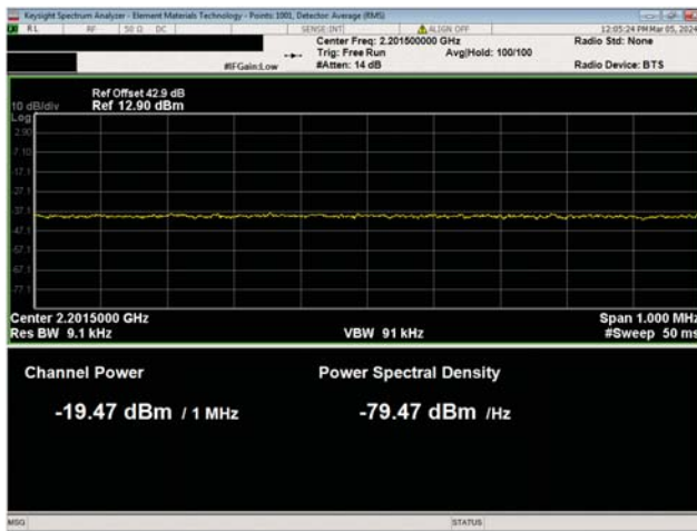
Band n66, 5G NR, 2110.0 MHz - 2200.0 MHz 35 MHz Channel Bandwidth 256QAM Modulation High Channel, 2182.5 MHz
