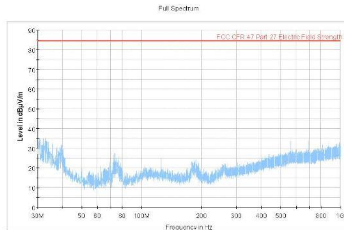
Figure 251 Radiated Emission 30 MHz – 1 GHz (2647.5MHz/2622.5MHz) (15MHz+15MHz Channel BW)
