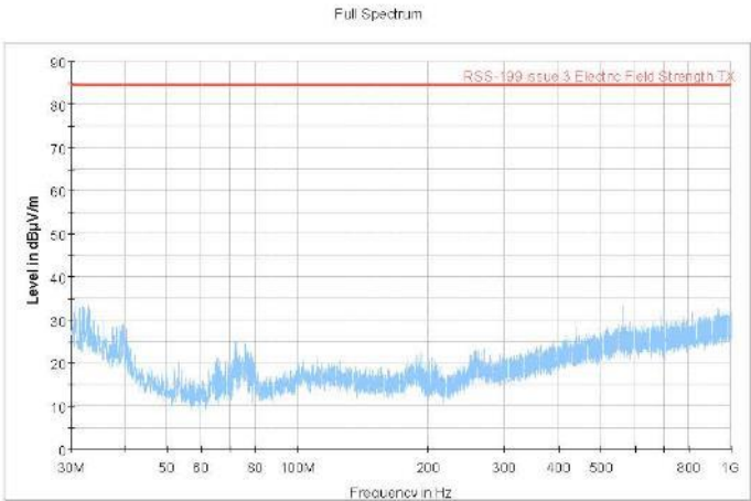
Figure 305 Radiated Emission 30 MHz – 1 GHz (2652.5/2657.5MHz) (5+5 MHz Channel BW)
