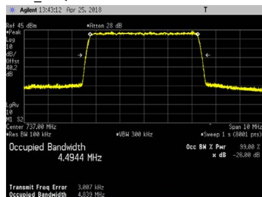
LTE5_64QAM
