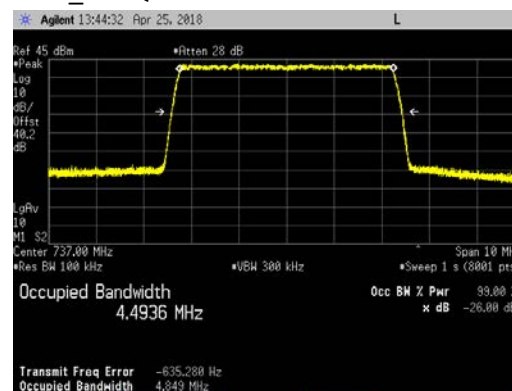
LTE5_256QAM
