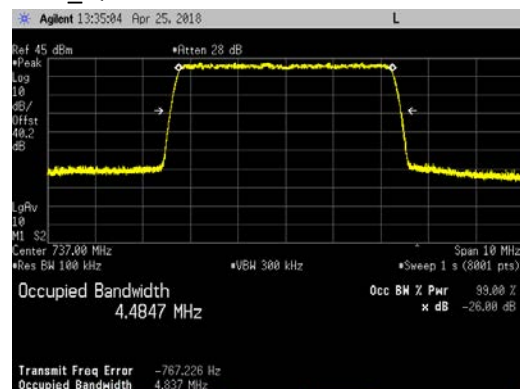
LTE5_QPSK
