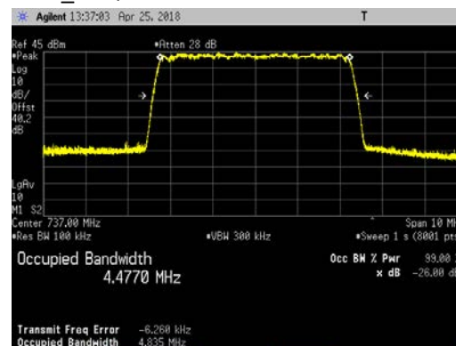
LTE5_16QAM
