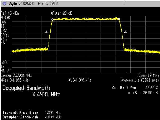
LTE5_64QAM
