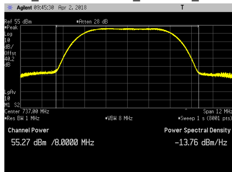
LTE5_ Middle Channel_256QAM_Peak
