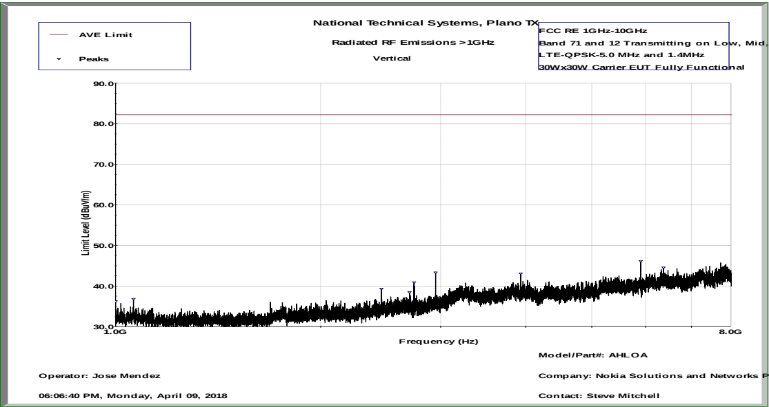
Radiated Spurious Emissions – 1-8GHz – Vertical Band 71 & 12
