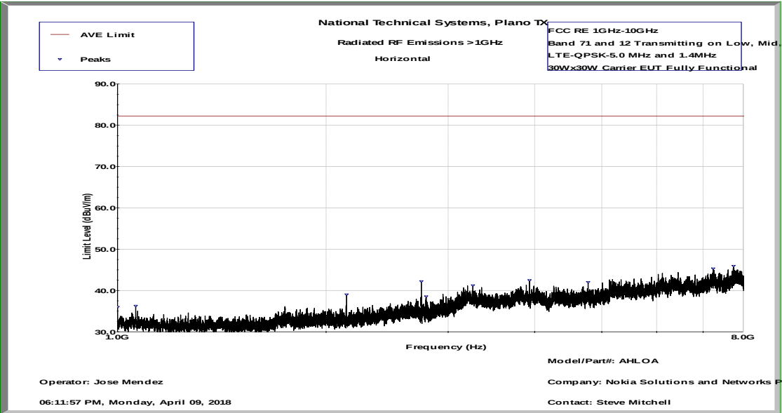
Radiated Spurious Emissions – 1-8GHz – Horizontal Band 71 & 12
