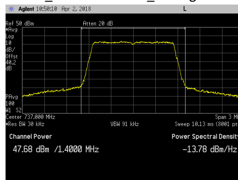
LTE1.4_Middle Channel_Average
