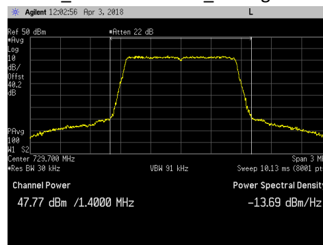
LTE1.4_Bottom Channel_Average
