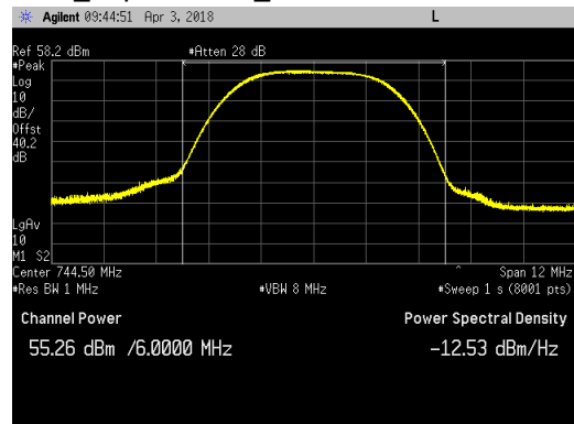
LTE3_Top Channel_Peak
