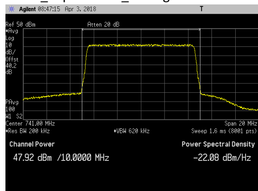
LTE10_Top Channel_Average
