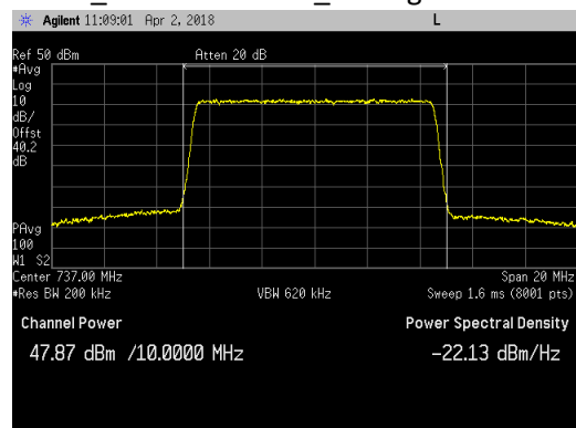
LTE10_Middle Channel_Average
