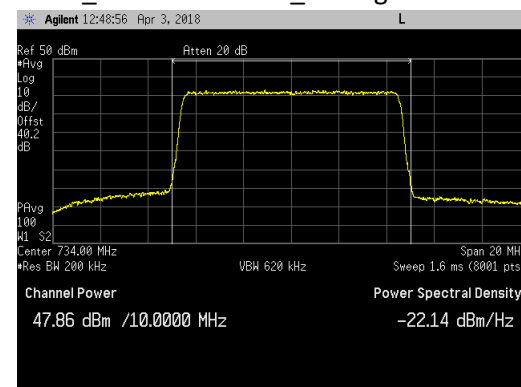
LTE10_Bottom Channel_Average
