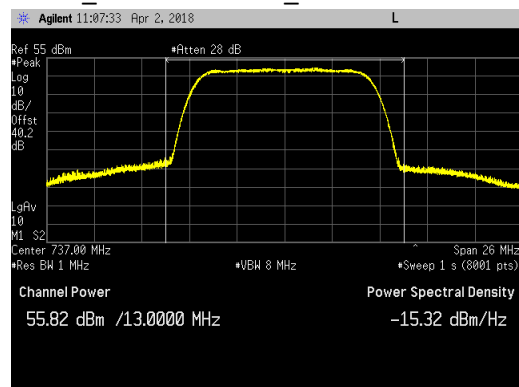
LTE10_Middle Channel_Peak
