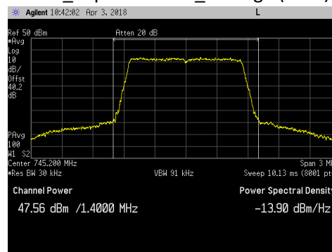
LTE1.4_Top Channel-1_Average (60W)
