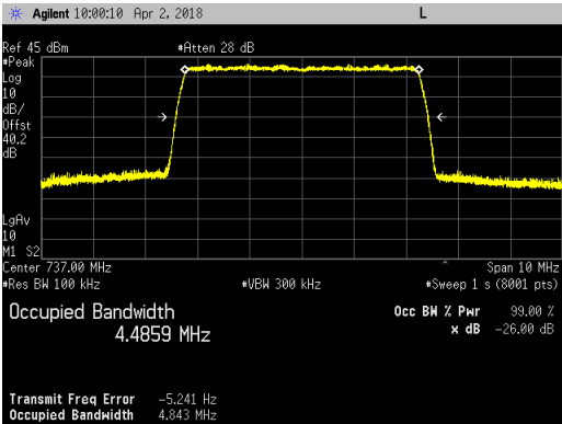
LTE5_QPSK
