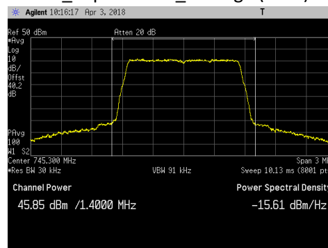
LTE1.4_Top Channel_Average (40W)
