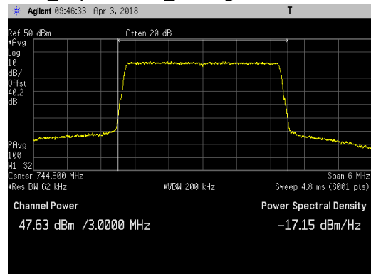
LTE3_Top Channel_Average
