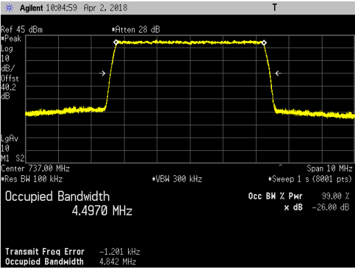
LTE5_256QAM
